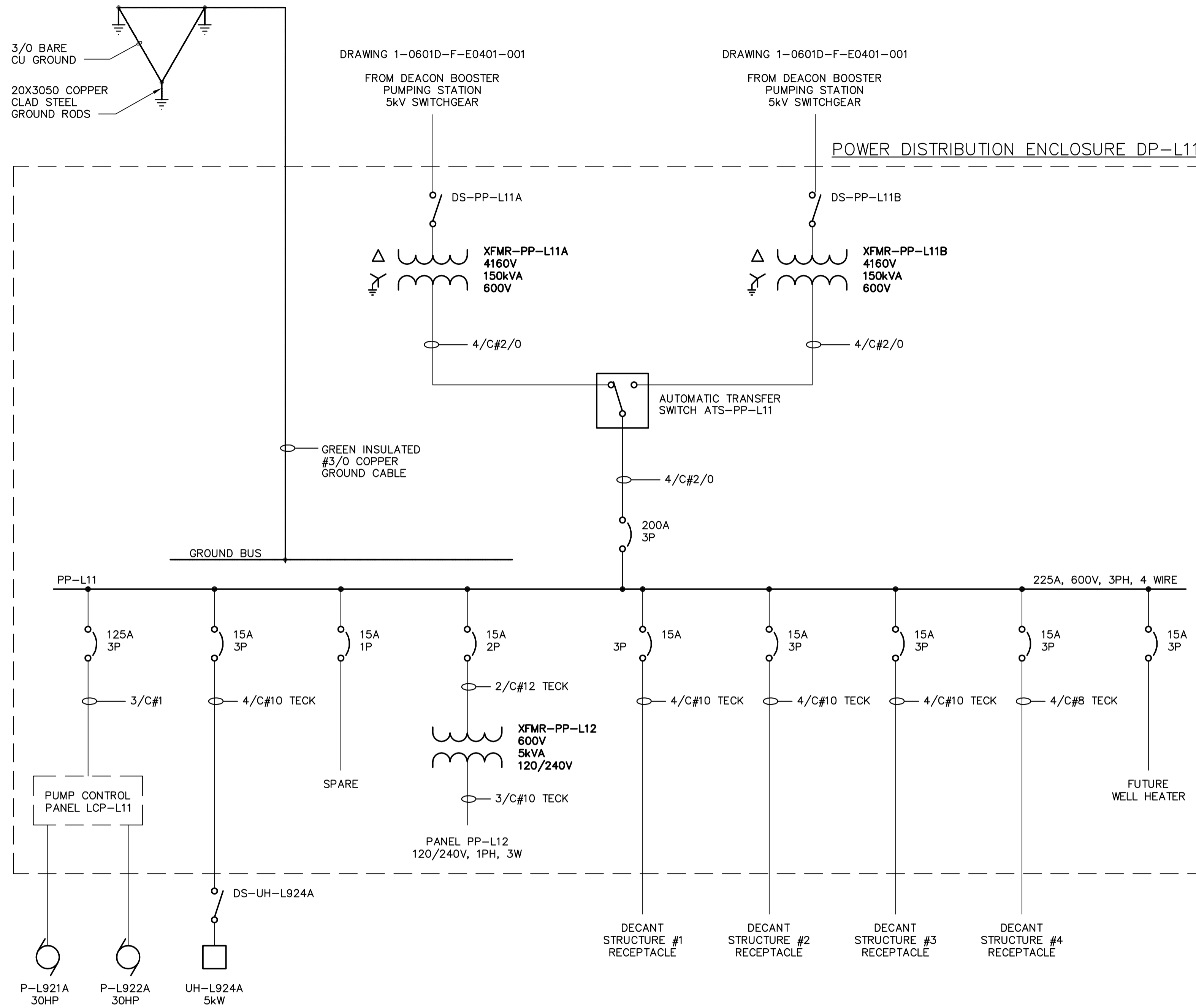
SINGLE LINE DIAGRAM NTS
