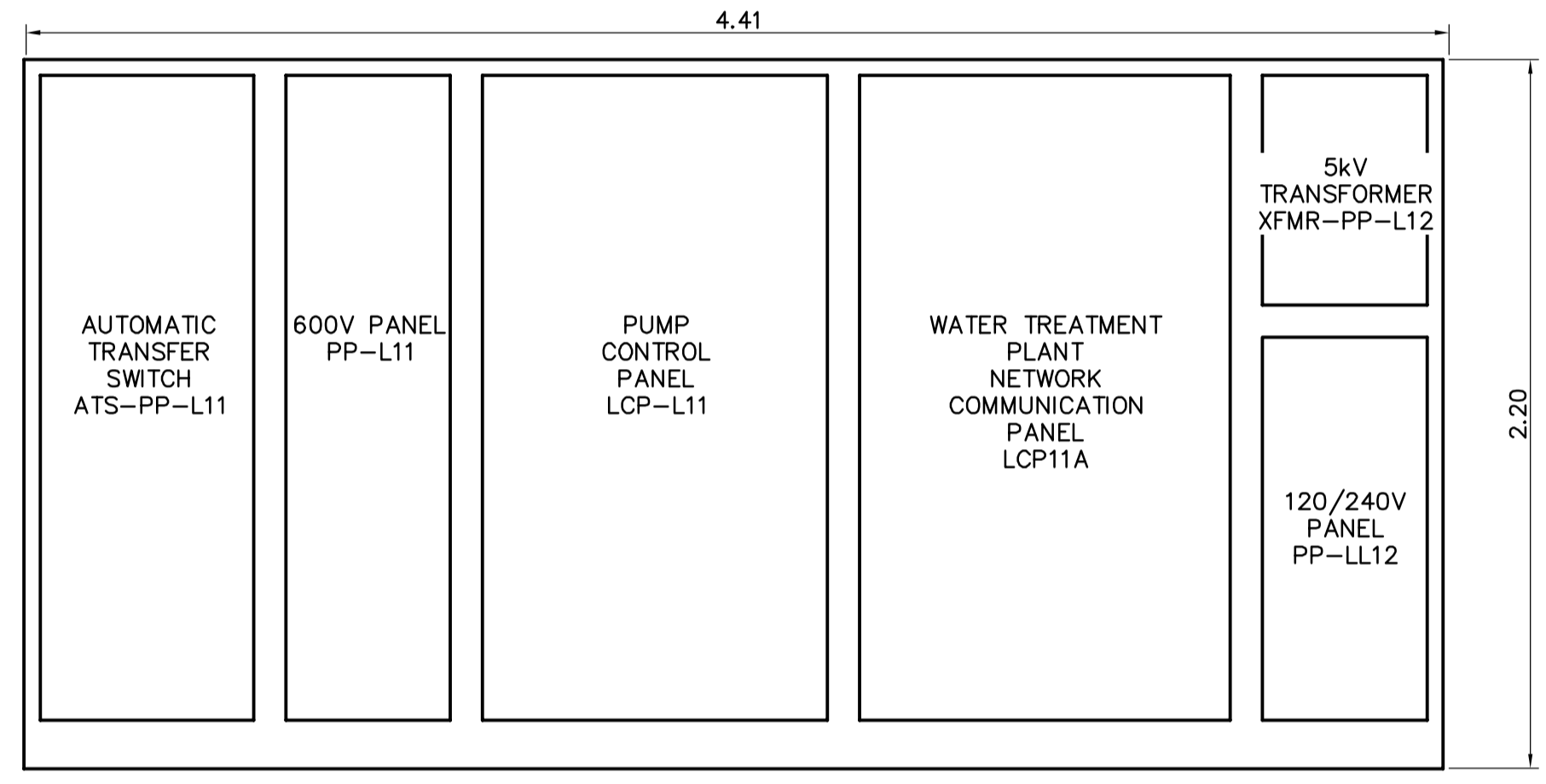
FRONT VIEW
