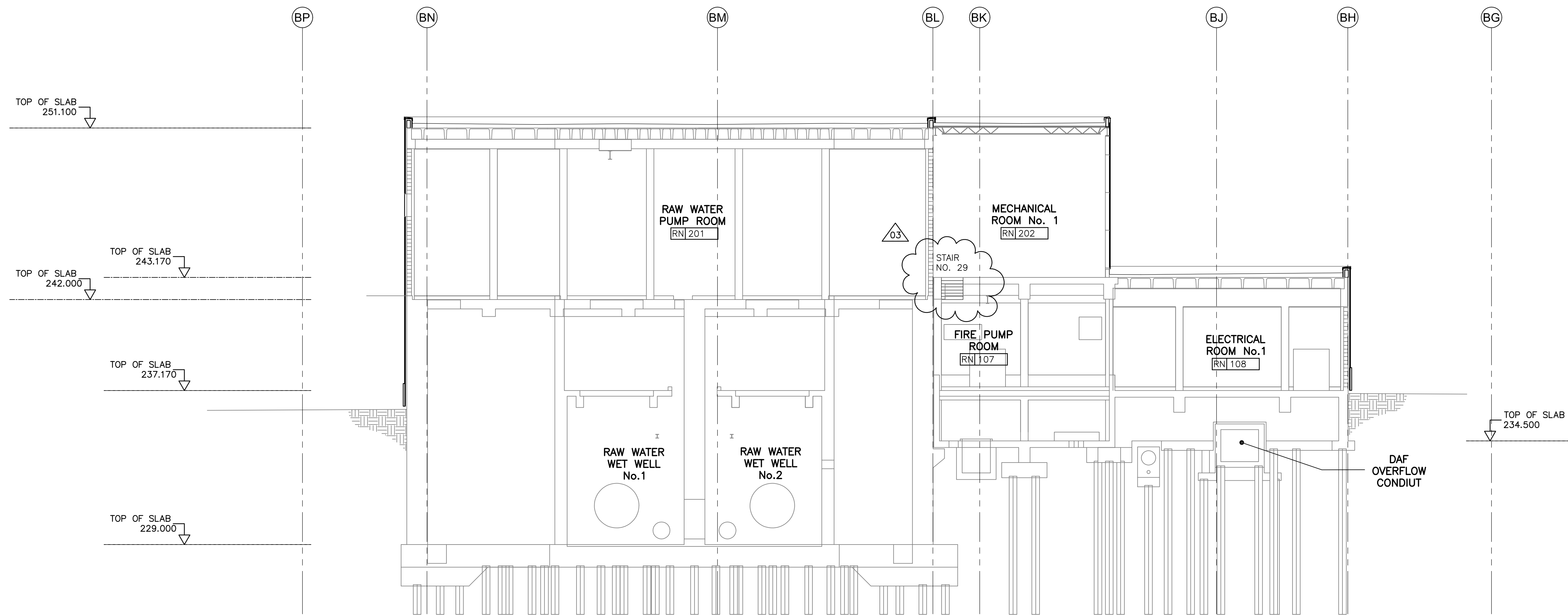
AA BUILDING SECTION SCALE 1:125
