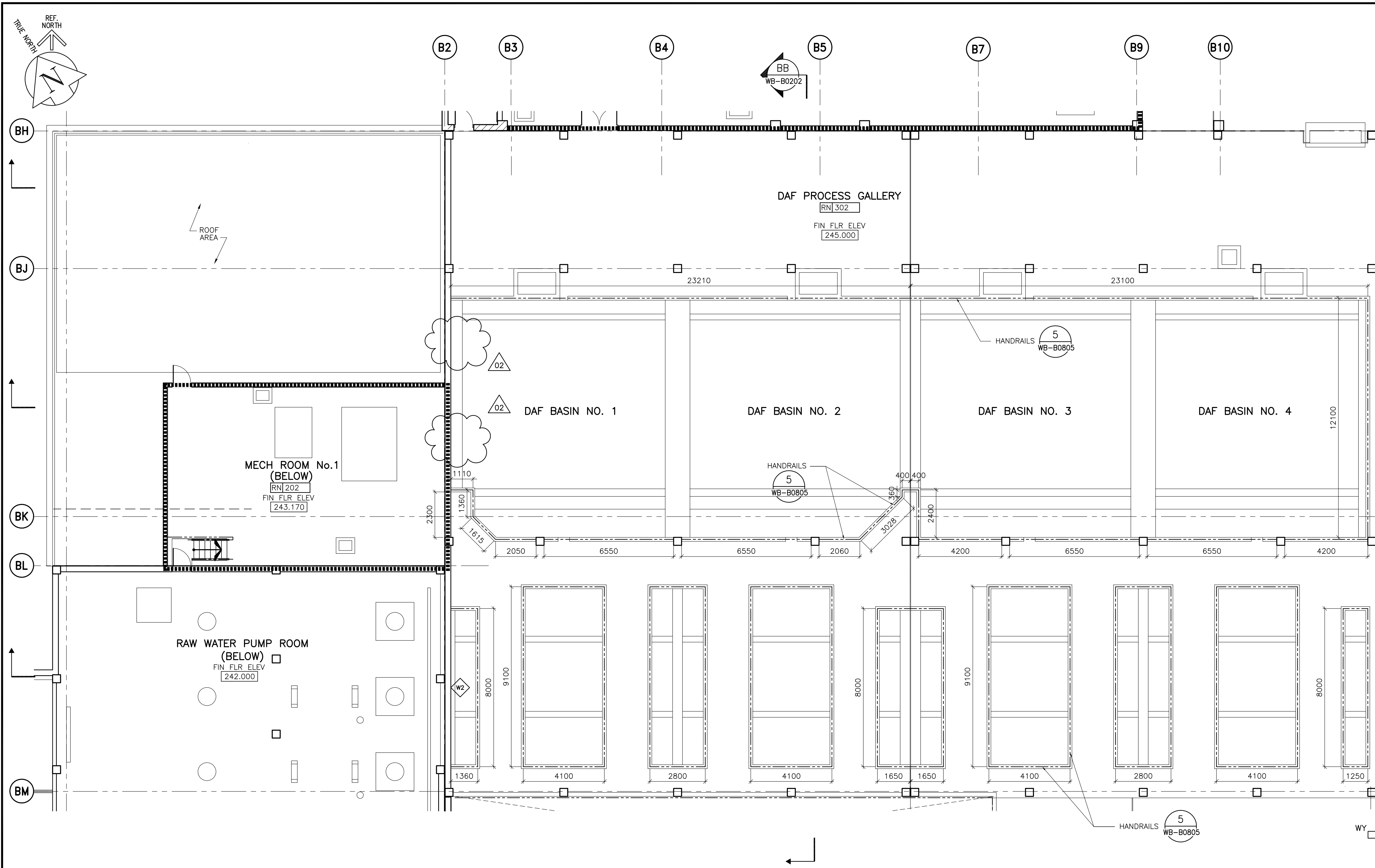
1 PARTIAL PLAN - DAF TANK & GALLERY AND MECH. ROOM #1 (THIRD FLOOR) WB-B0136 1:100
