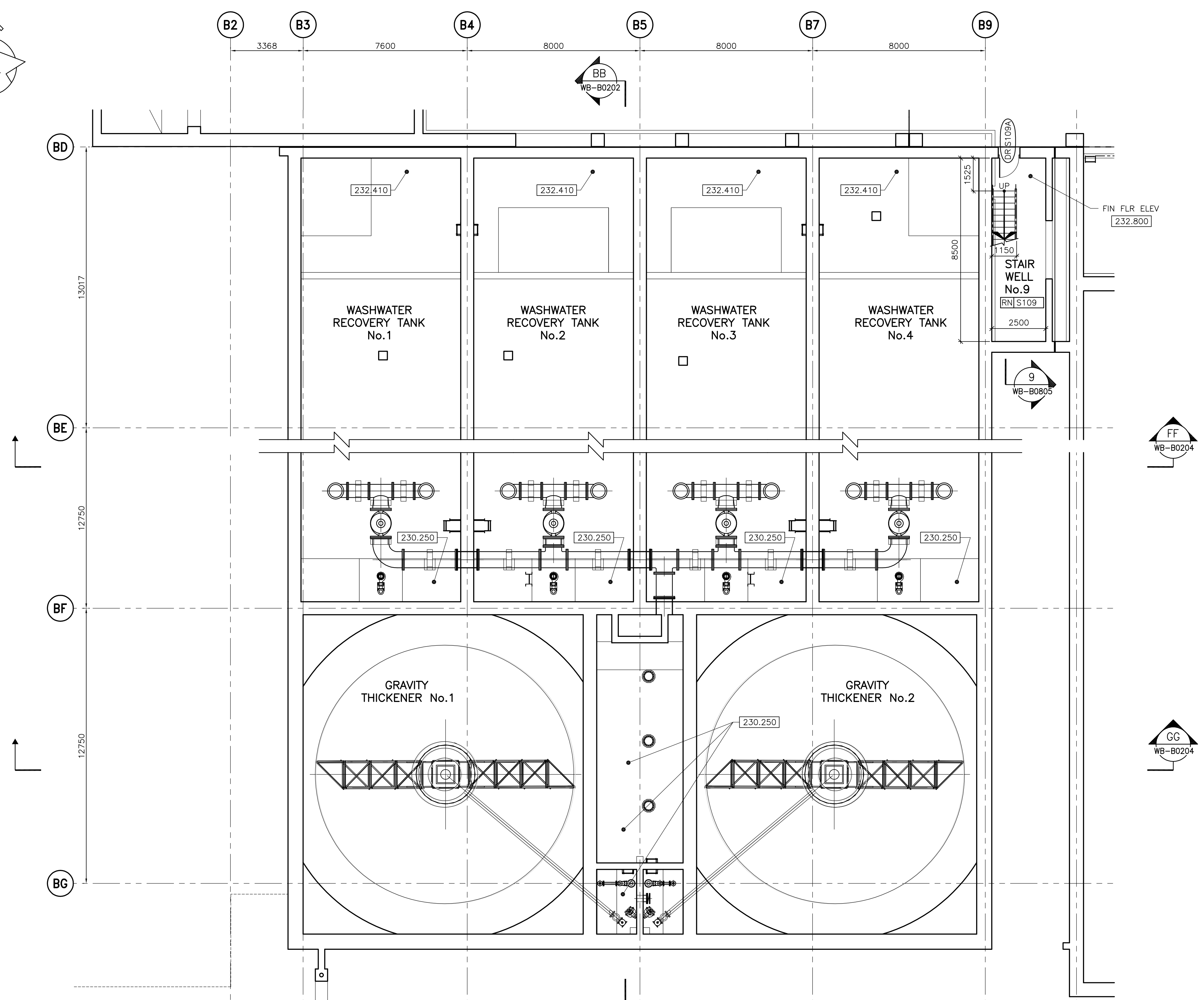
1 PARTIAL PLAN - RESIDUAL TANK AREA (LOWER LEVEL) WB-B0103 1:100
