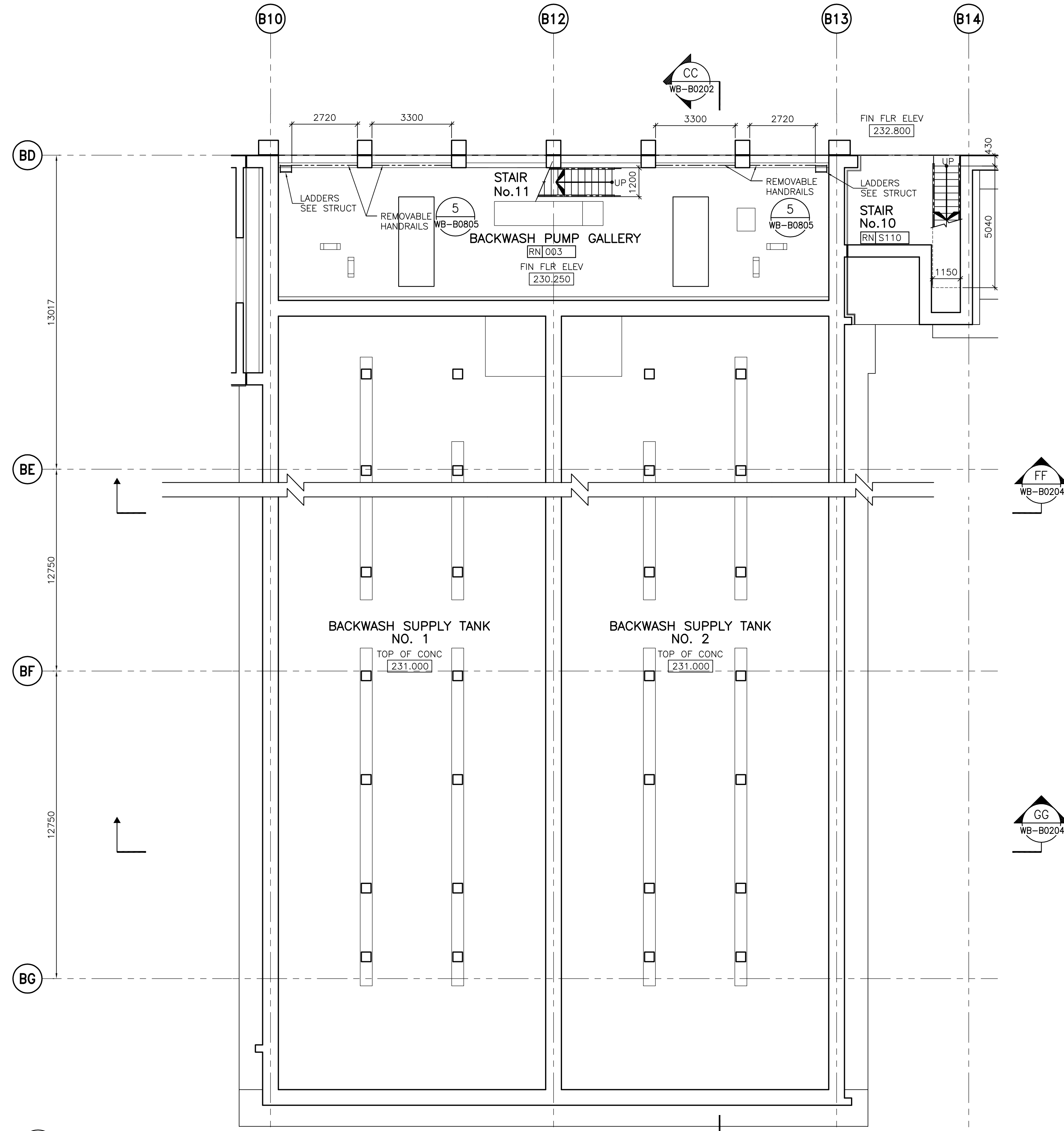
1 PARTIAL PLAN - BACKWASH SUPPLY TANKS AND PUMP GALLERY (LOWER LEVEL) WB-B0104 1:100
