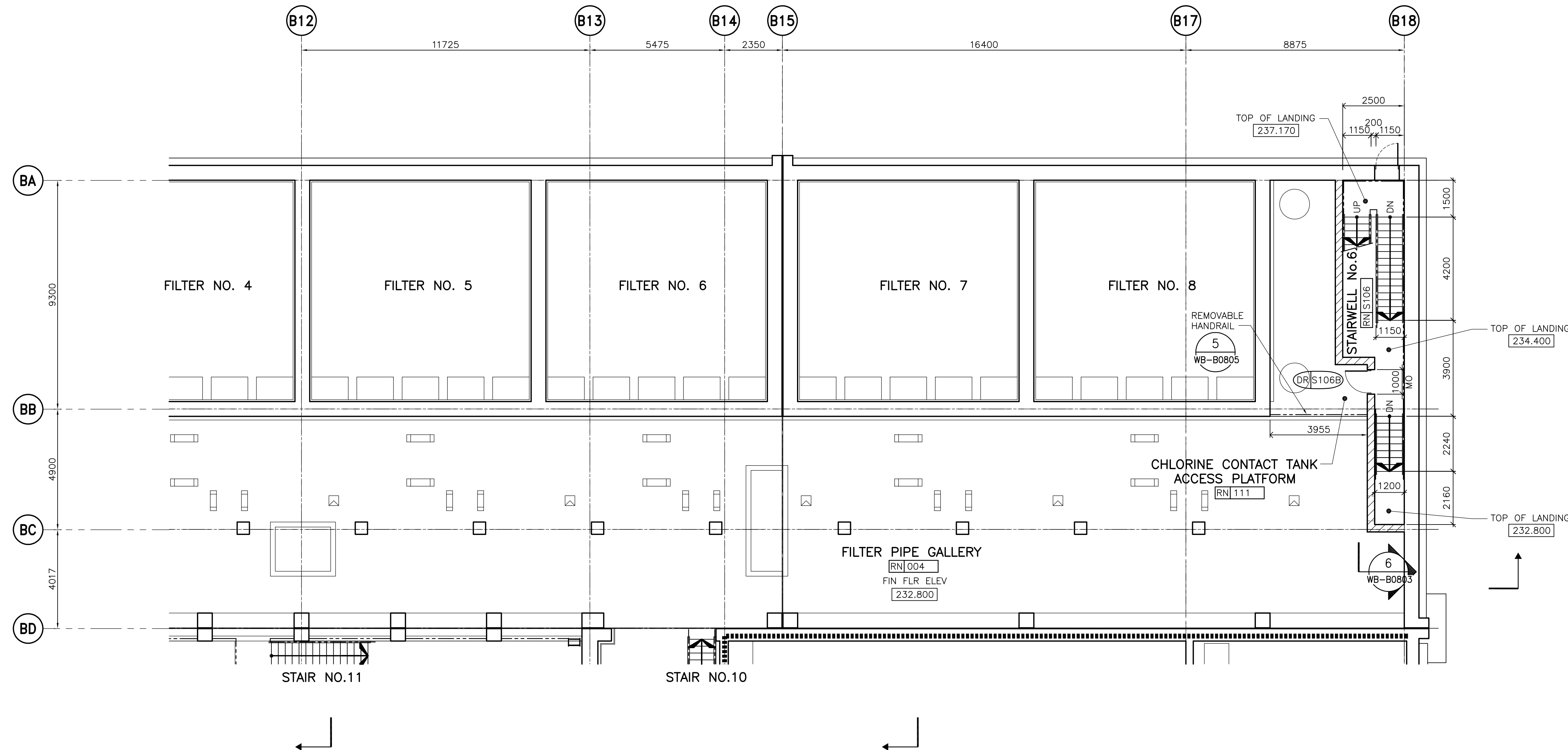
1 PARTIAL PLAN - FILTER CHANNEL & GALLERY (FIRST FLOOR LEVEL) WB-B0112 1:100
