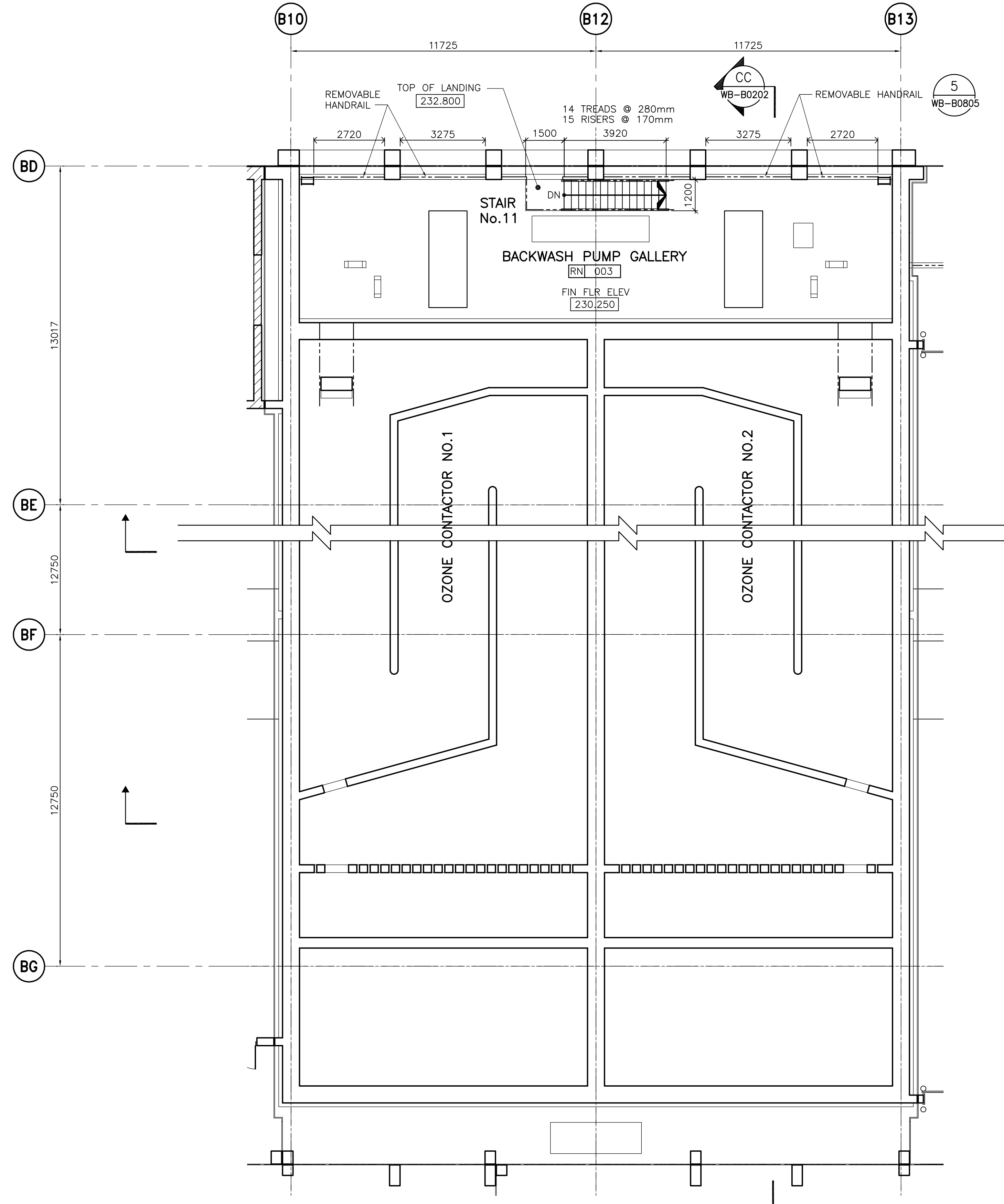
1 PARTIAL PLAN - OZONE TANK, & BACKWASH PUMP GALLERY (FIRST FLOOR) WB-B0114 1:100
