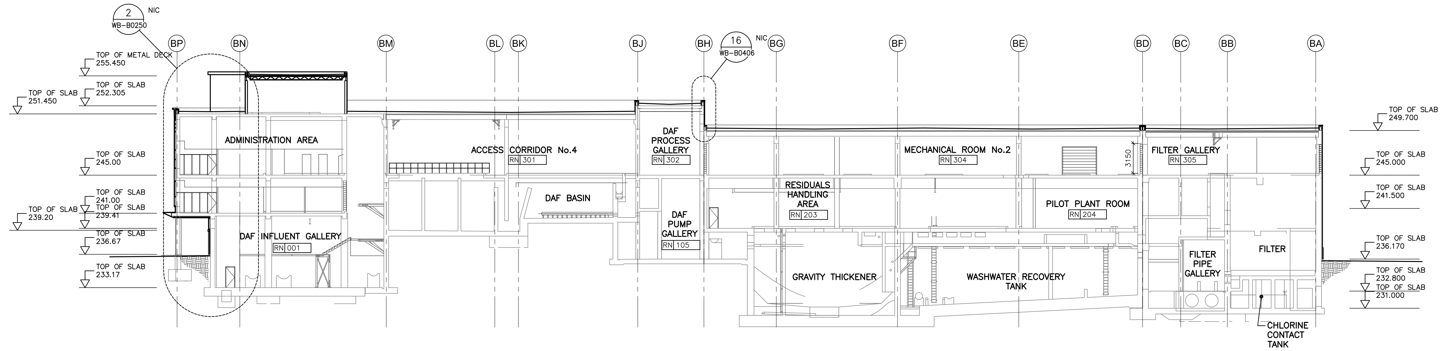
BB BUILDING SECTION SCALE 1:200
