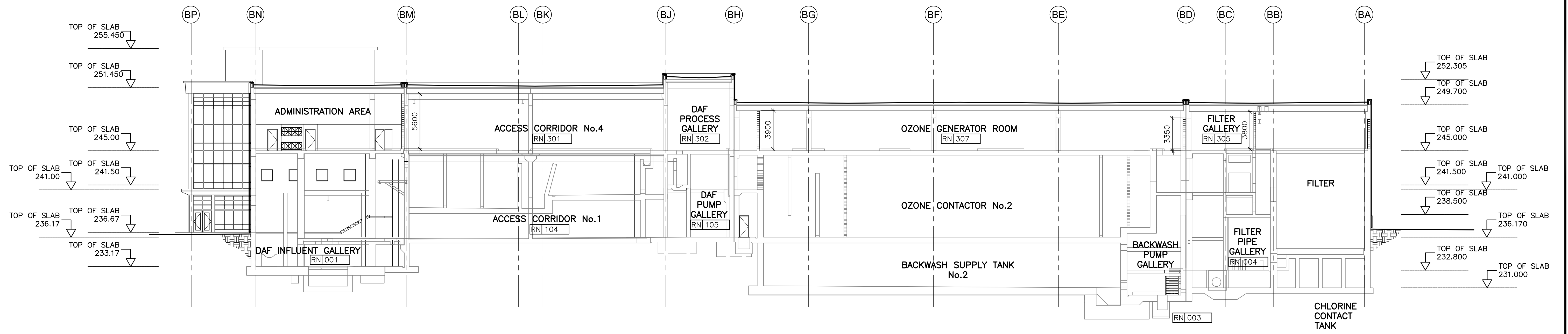
CC BUILDING SECTION SCALE 1:200
