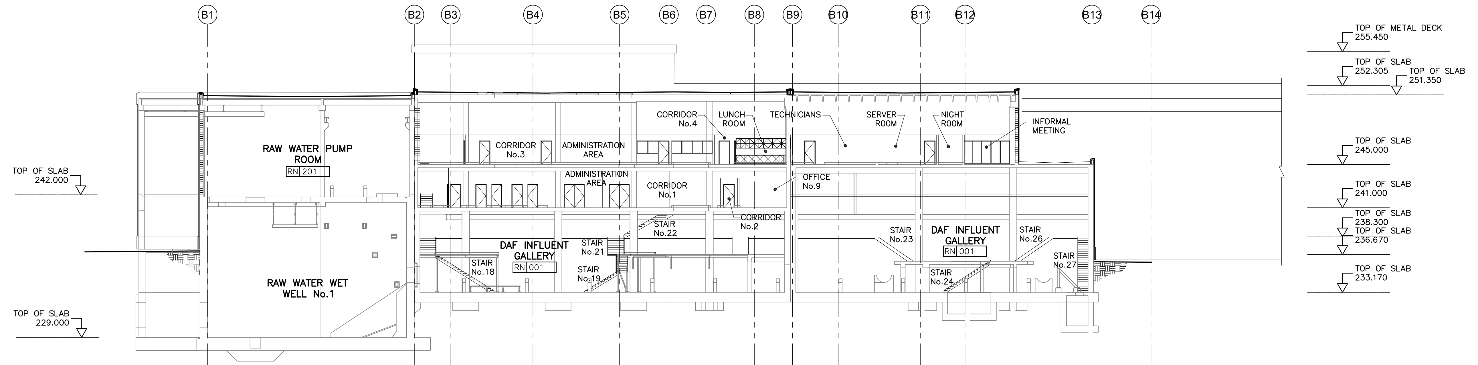
MM BUILDING SECTION SCALE 1:200
