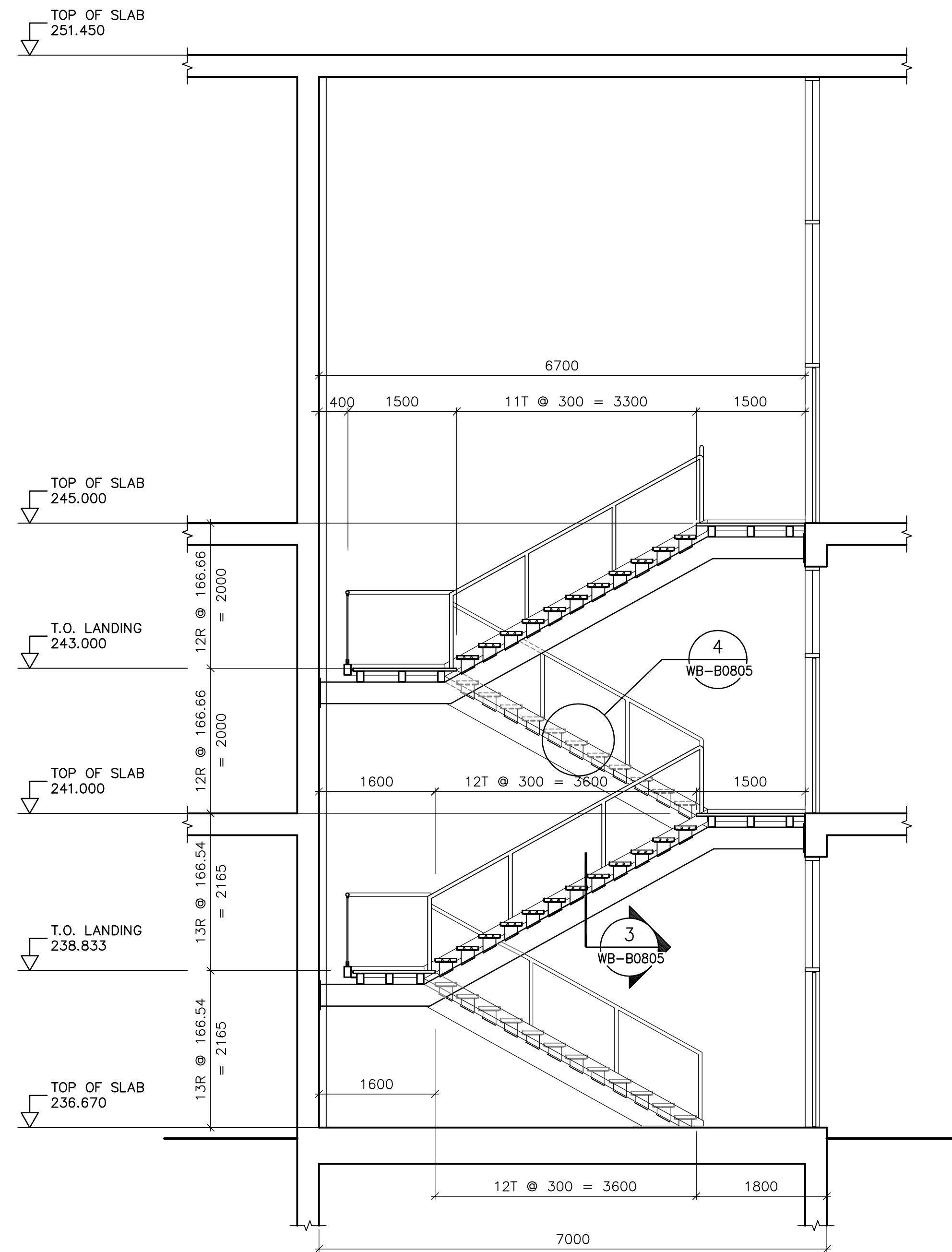
1 STAIRWELL NO.1 SECTION DETAIL WB-B0119 1:50
