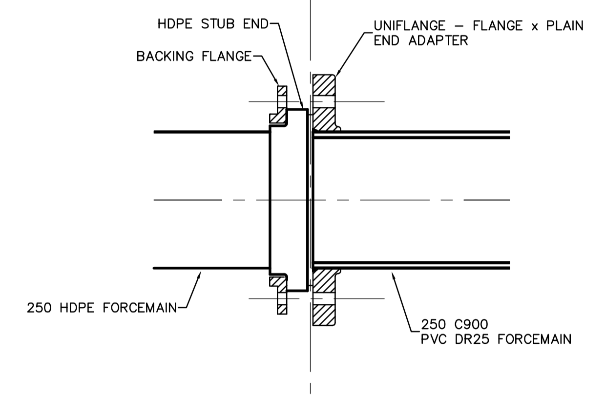
2 HDPE TO PVC CONNECTION WZ-C0118 NTS
