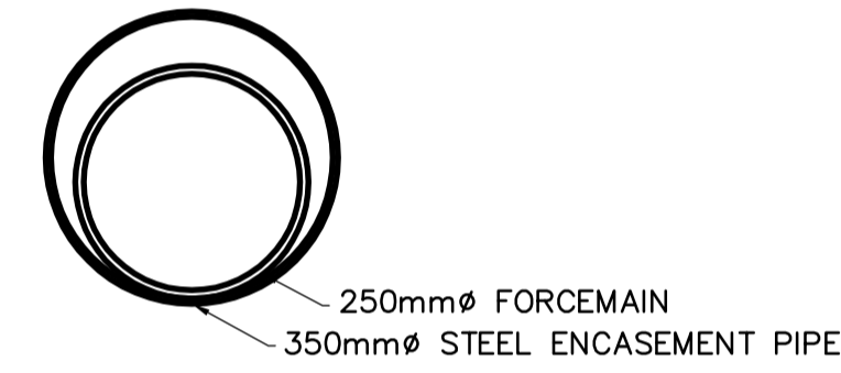
1 CASING PIPE DETAIL WZ-C0101 NTS
