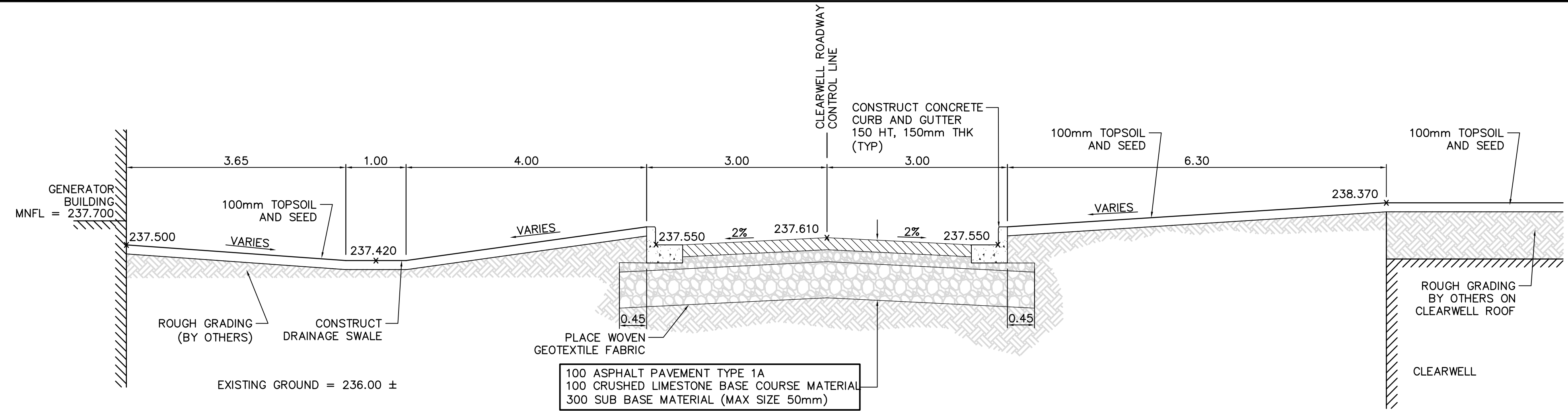
7 SECTION AT CLEARWELL ROADWAY STA 0+440 C0163 SCALE H=1:50 V=1:25
