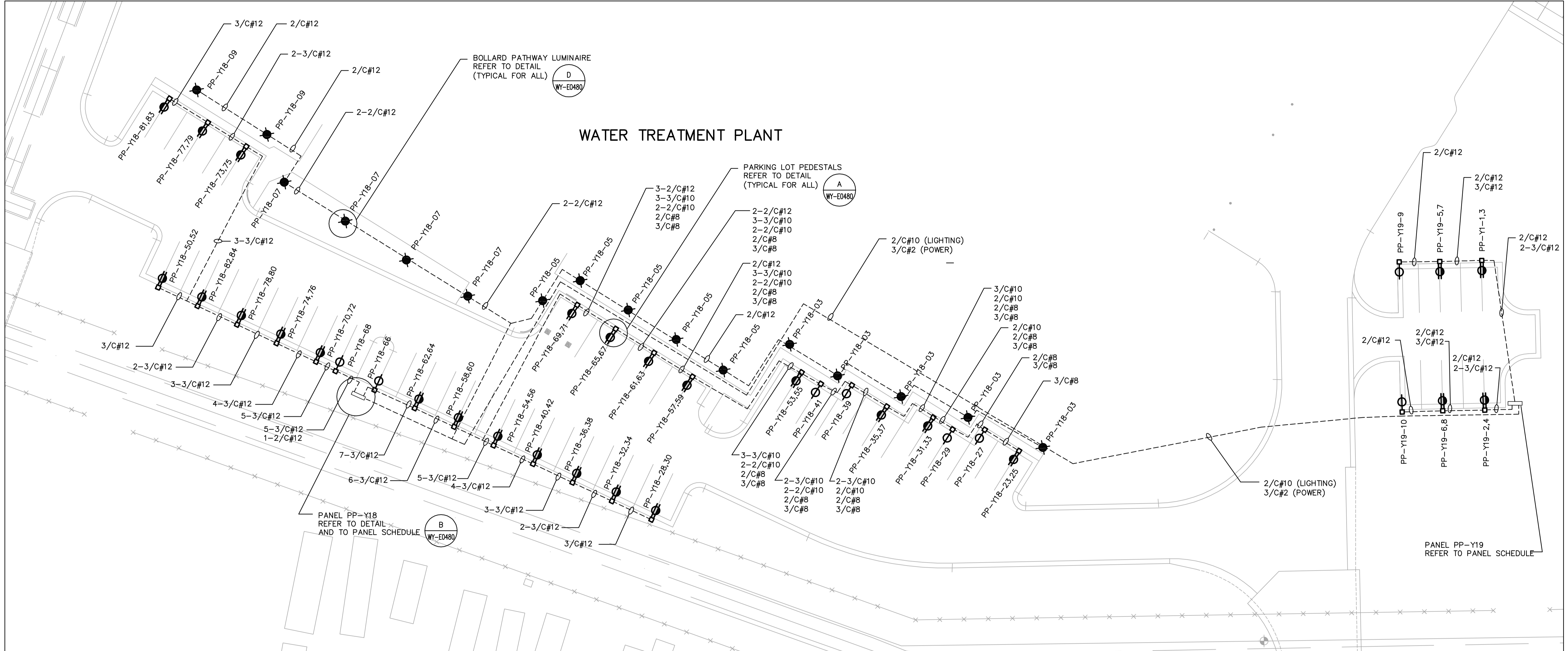
PARKING LOT POWER PLAN SCALE: 1 : 250
