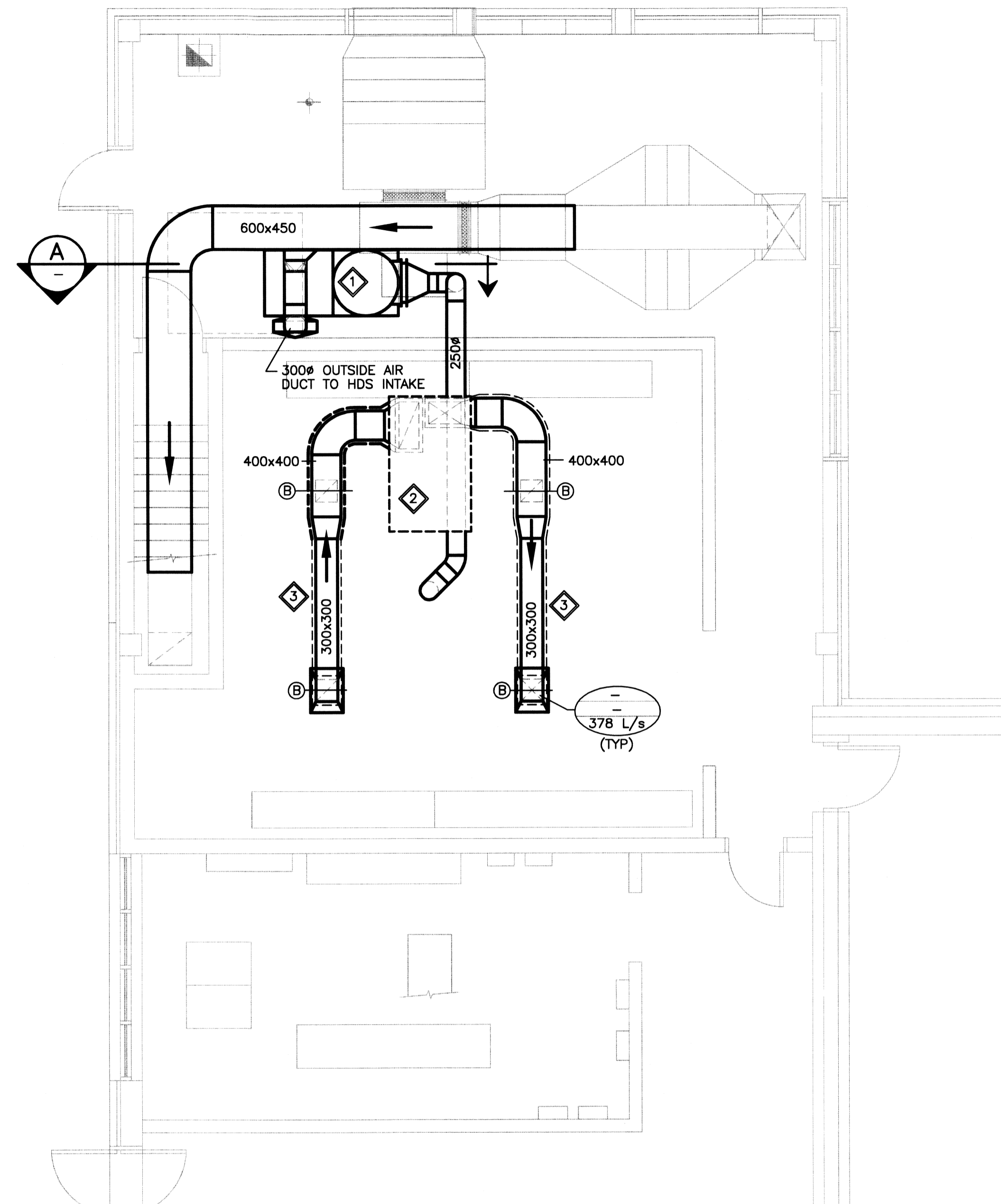
1 CLARIFIER ELECTRICAL ROOM PLAN - NEW VENTILATION
