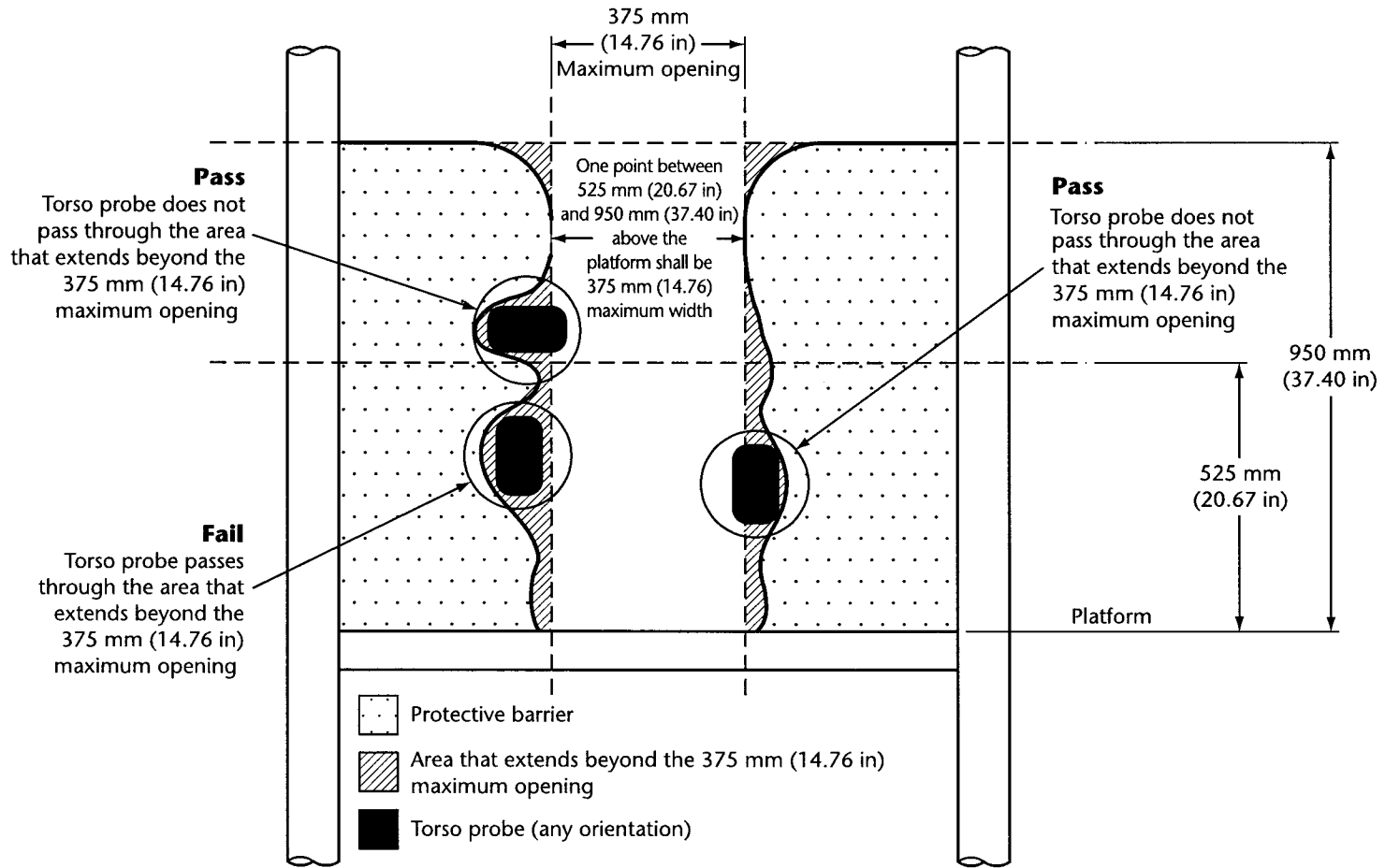
Figure 20 Guardrail or protective barrier openings
