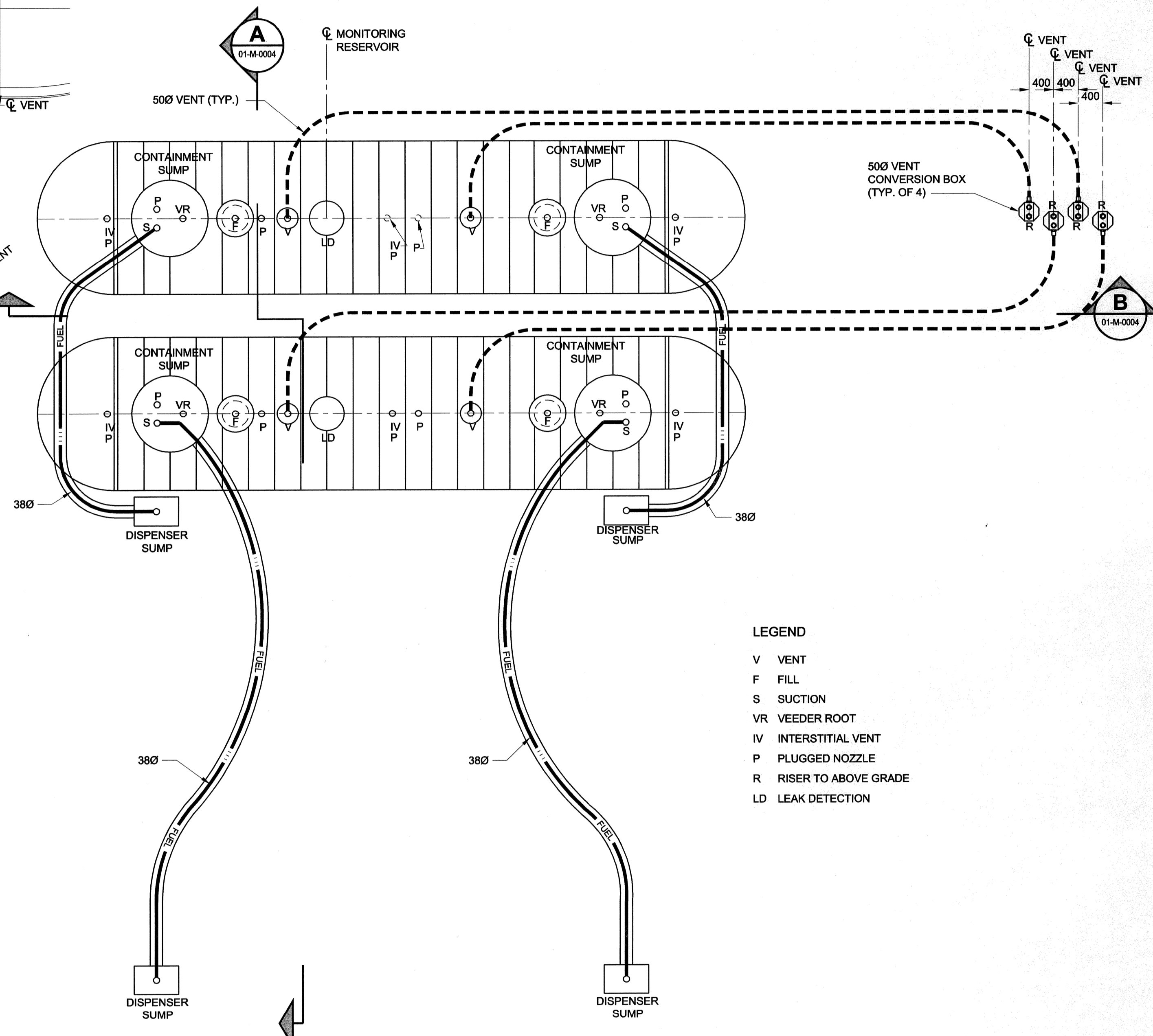
PLAN 2 SCALE 1:50 0 500 1000 1500 mm BELOW GRADE
