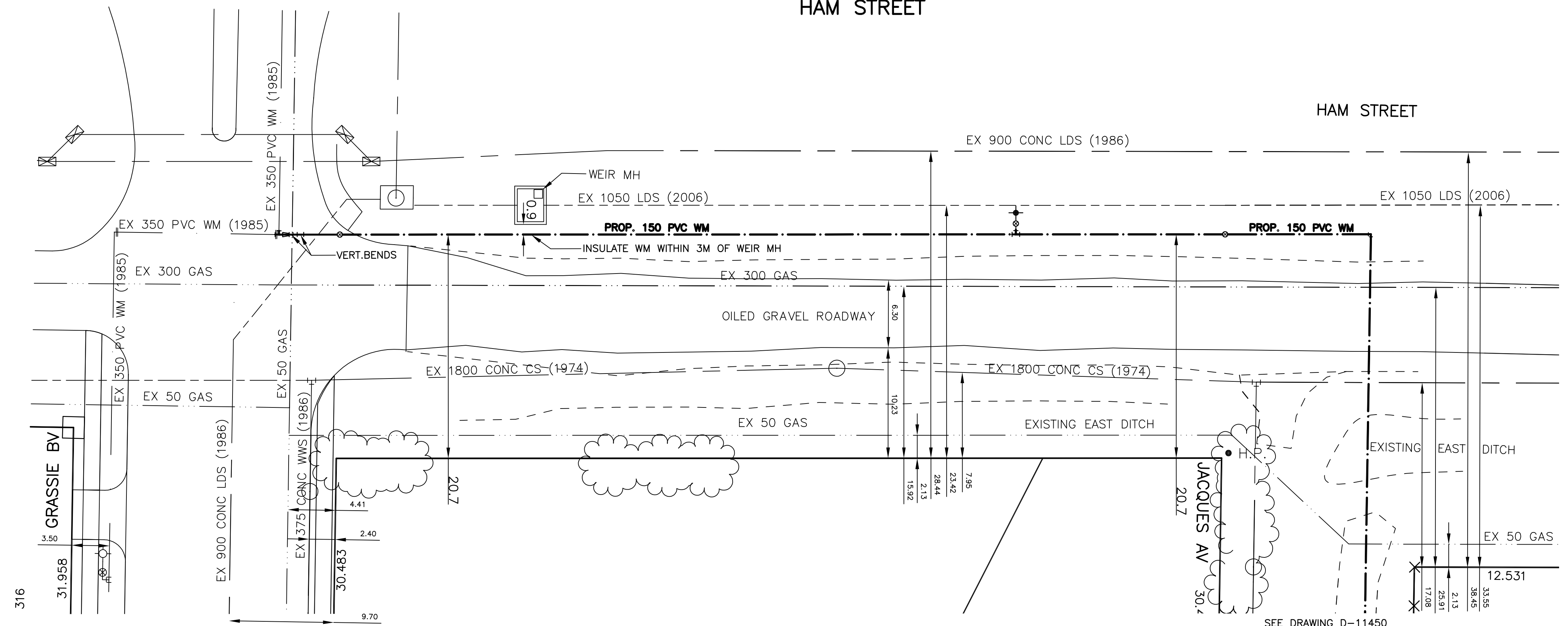
CHAINAGE ALONG EAST PROPERTY LINE OF HAM STREET
