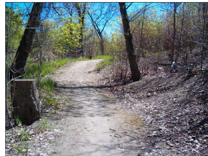
PHOTOGRAPH 15: FACING SOUTH - AT STATION 2+35, AREA WITH NO RETAINING WALL
