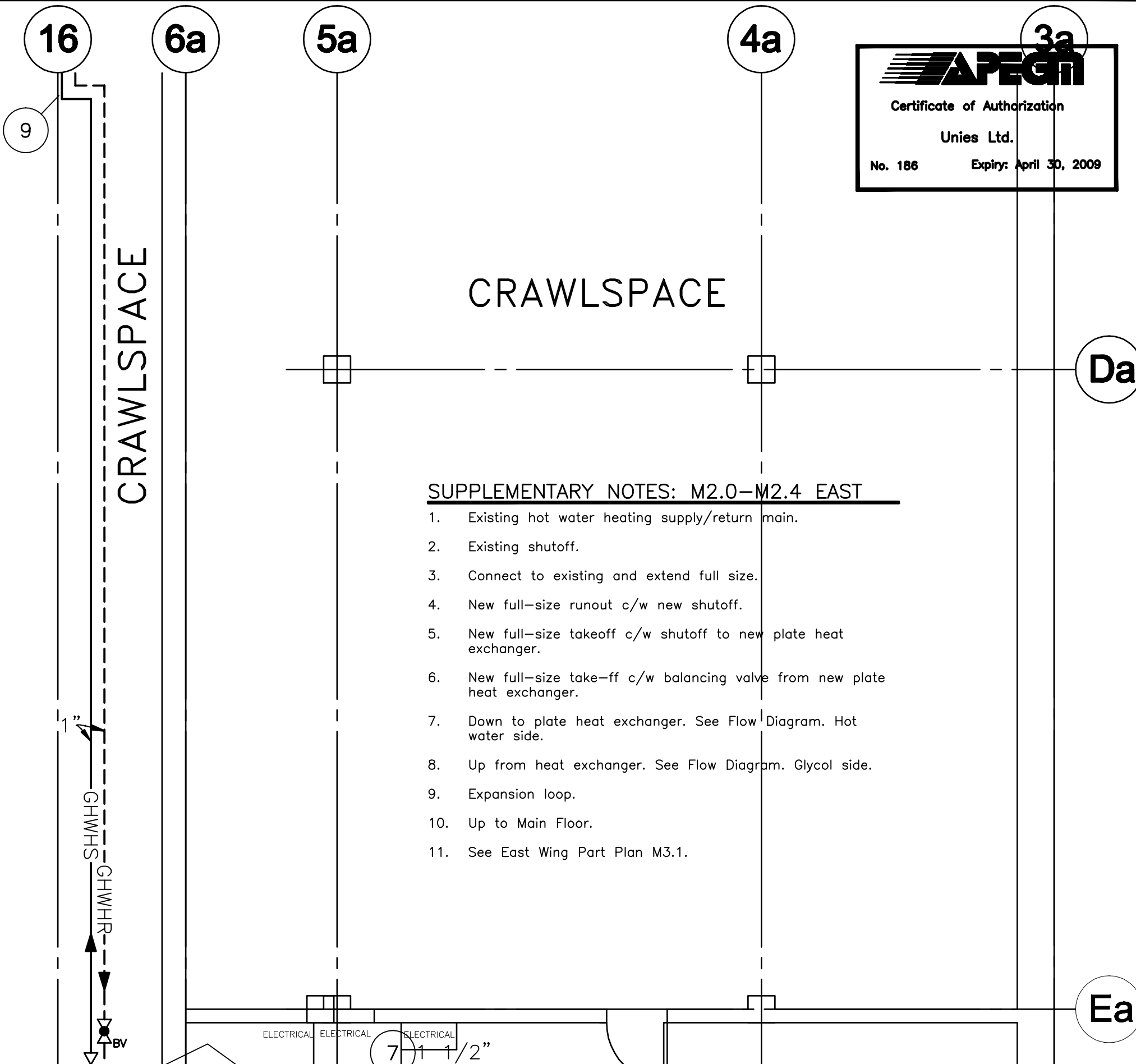
PART BASEMENT FLOOR PLAN NO.3 - NEW WORK SCALE: 3/16" = 1'-0"
