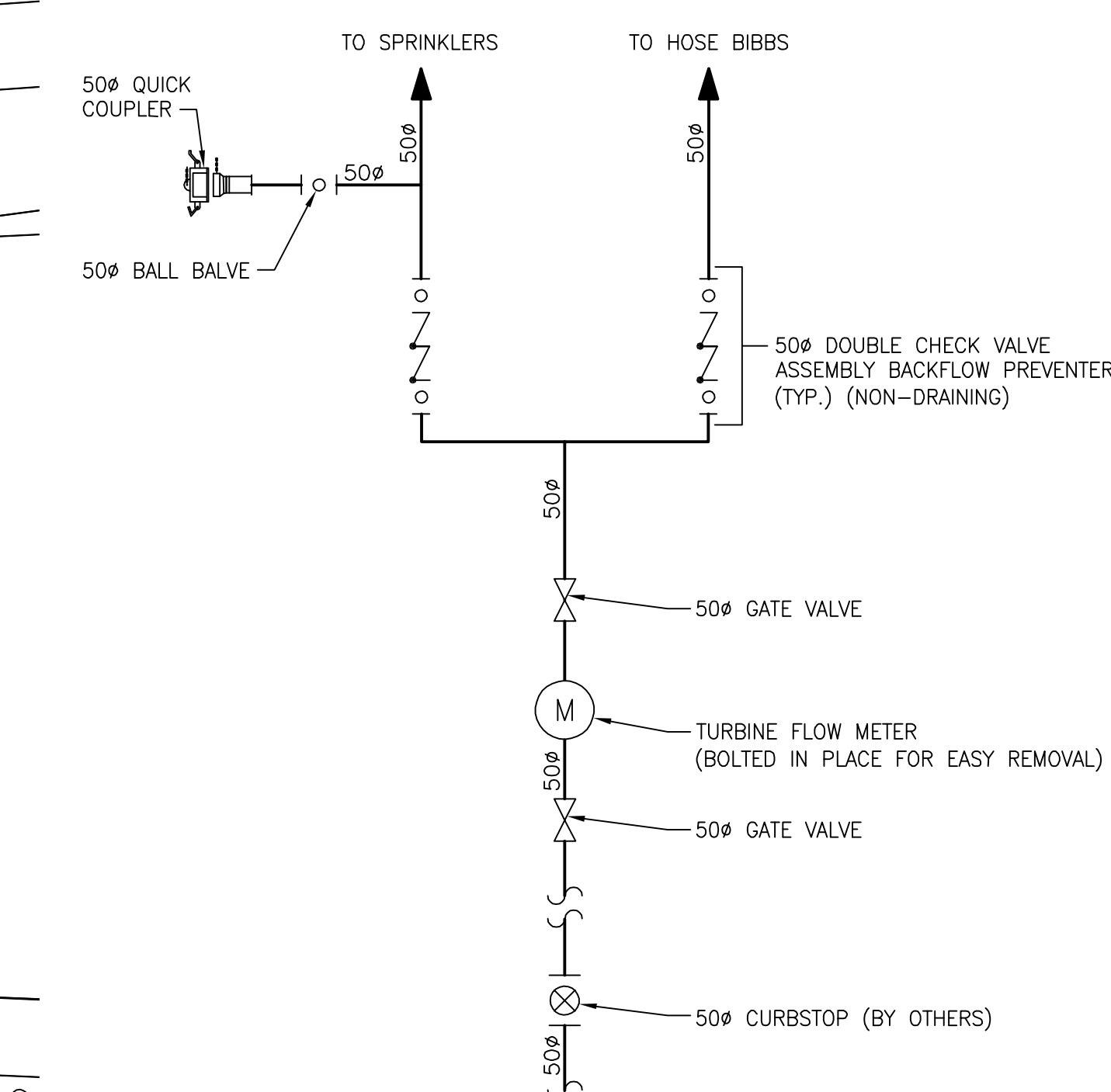
WATER SERVICE DISTRIBUTION SYSTEM
