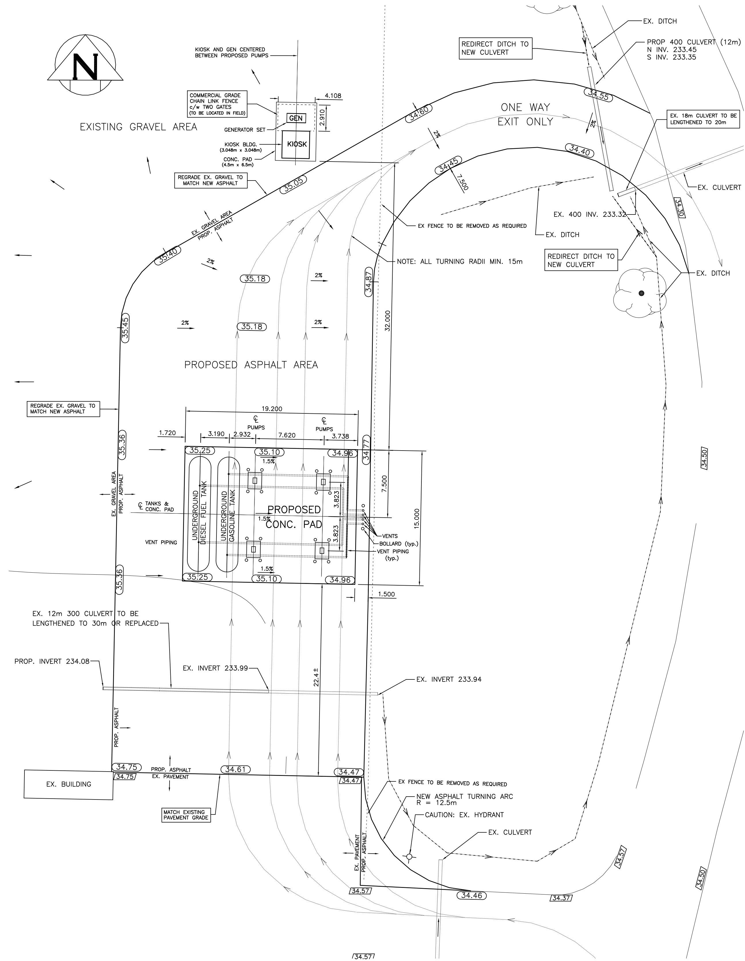
PAD AND NEW APPROACH DETAIL SCALE 1:250
