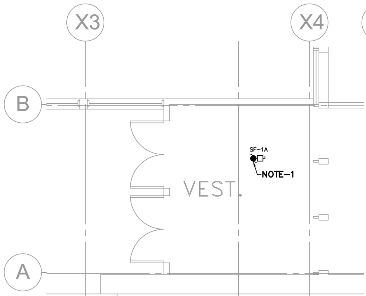
1 SOUTH/WEST VEST. PLAN - ELECTRICAL E2.3 SCALE: 3/16"=1'-0"
