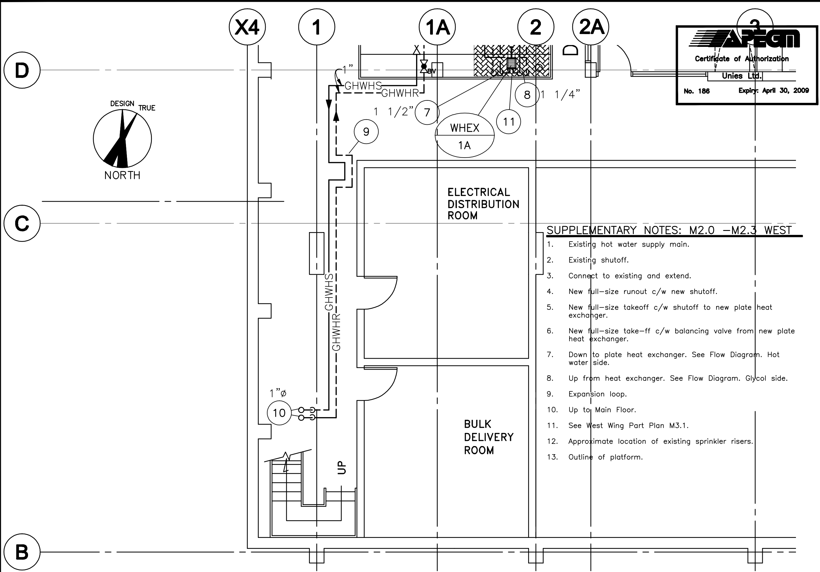
PART BASEMENT FLOOR PLAN NO.1 - NEW WORK SCALE: 3/16" = 1'-0"
