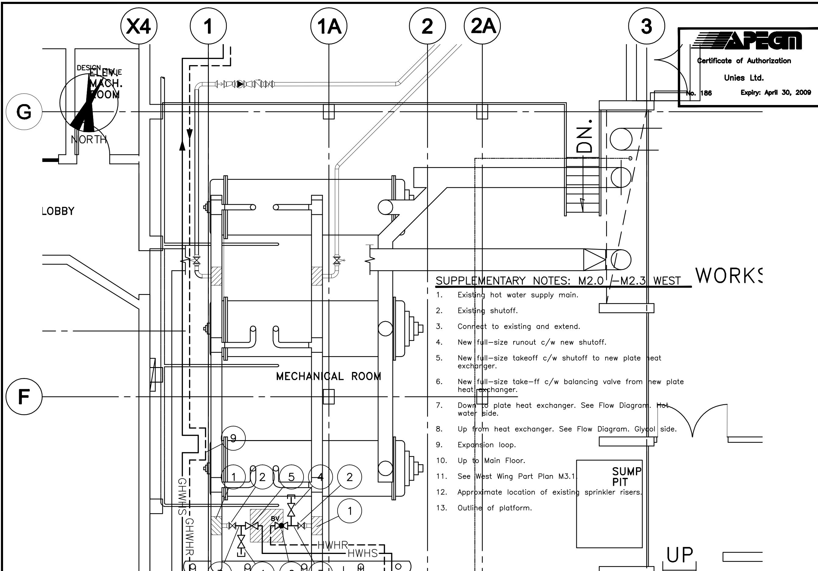
PART BASEMENT FLOOR PLAN NO.3 - NEW WORK SCALE: 3/16" = 1'-0"
