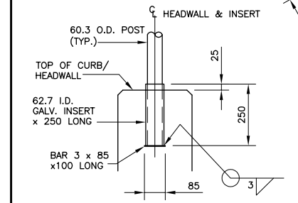
TYPICAL POST INSERT DETAIL 1: 10 (AT PROPOSED CONCRETE HEADWALL)
