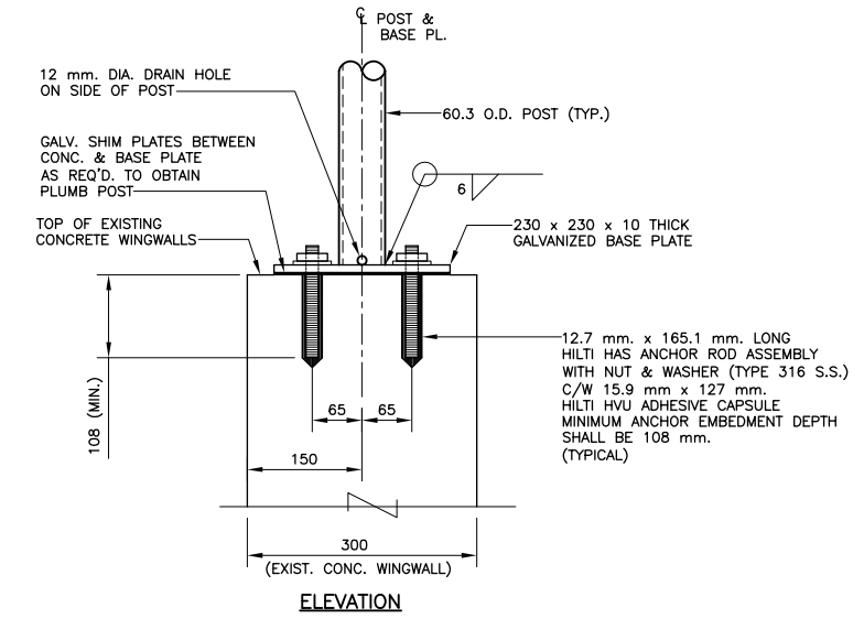
TYPICAL FENCE POST DETAIL 1: 5 (AT EXISTING WINGWALL)
