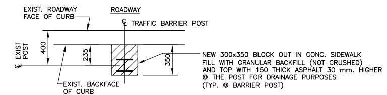
TYPICAL BARRIER POST BLOCK-OUT DETAIL 1: 20
