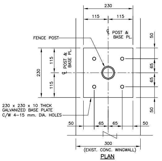
TYPICAL FENCE POST DETAIL 1: 5 (AT EXISTING WINGWALL)
