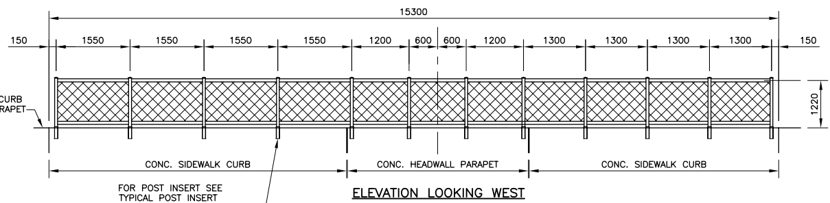
PROPOSED CHAINLINK FENCE EAST END OF CULVERT AT NEW CONCRETE HEADWALL 1: 50
