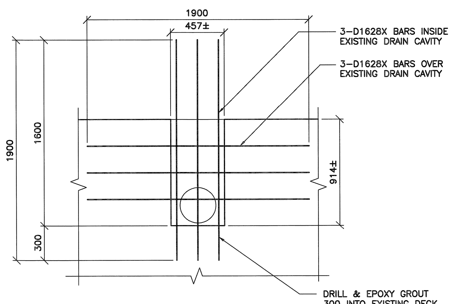
2 - - DETAIL 'A' 1 : 20 TYPICAL REINF. OVER EXISTING DRAINS (10 LOC'NS THUS)
