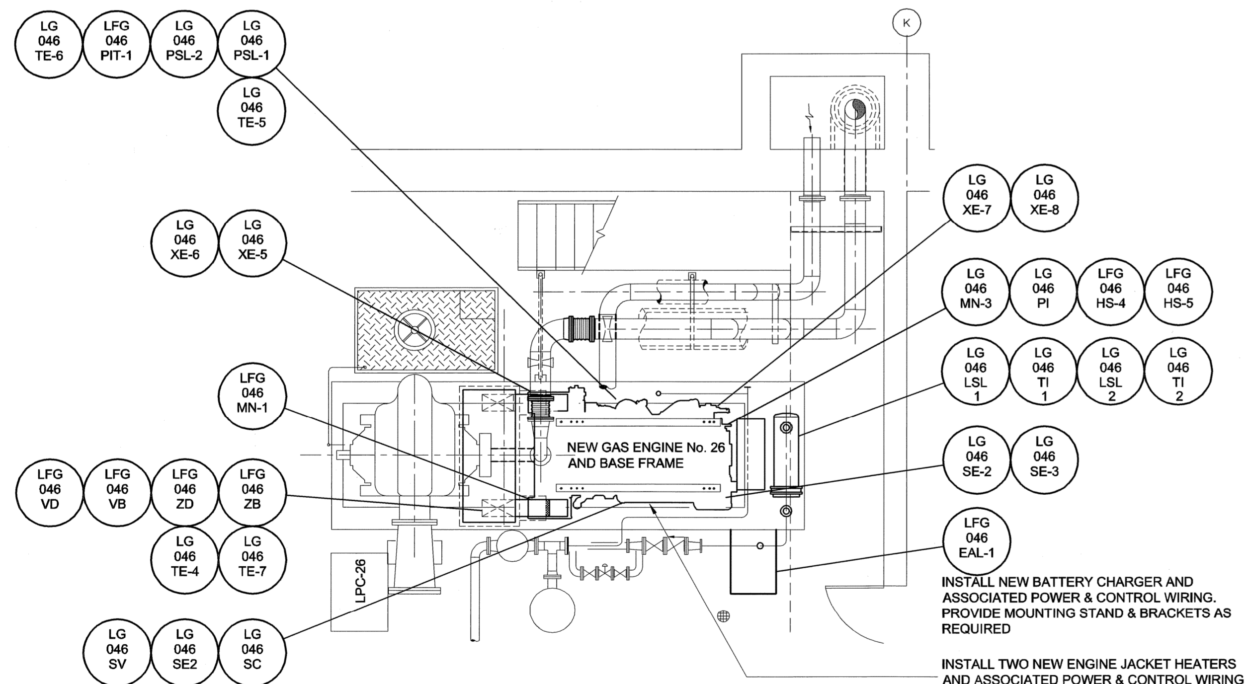
DETAIL P-26 SCALE 1:50 0 500 1000 1500 mm
