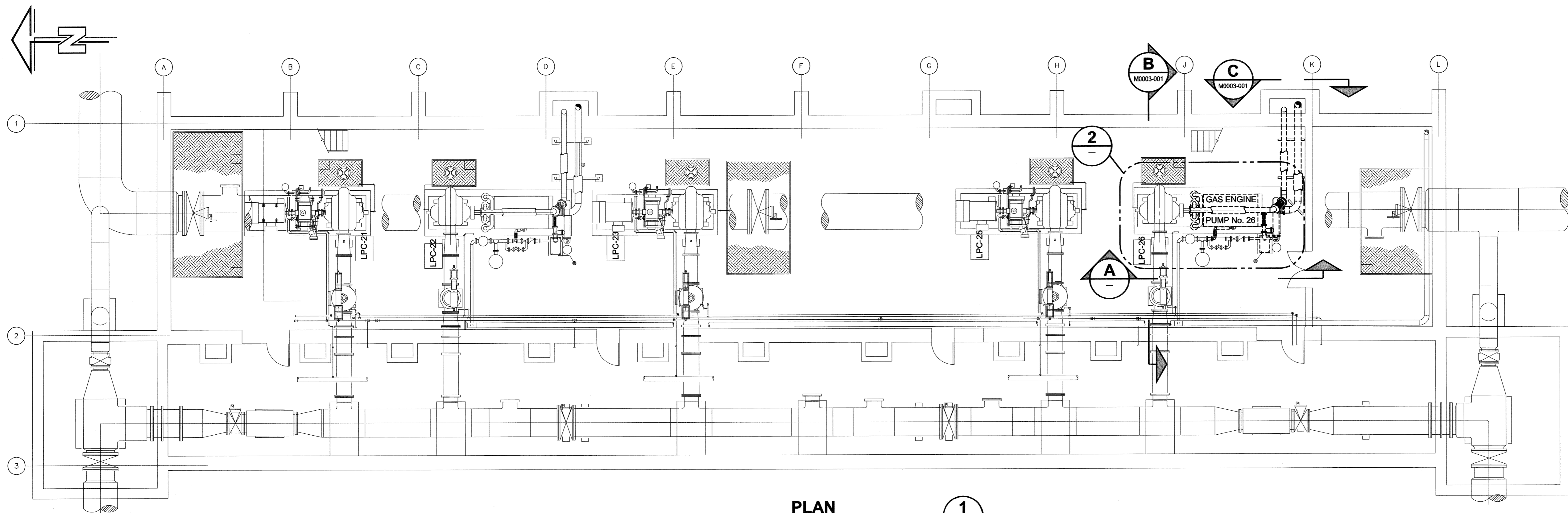
PLAN SCALE 1:100 1
