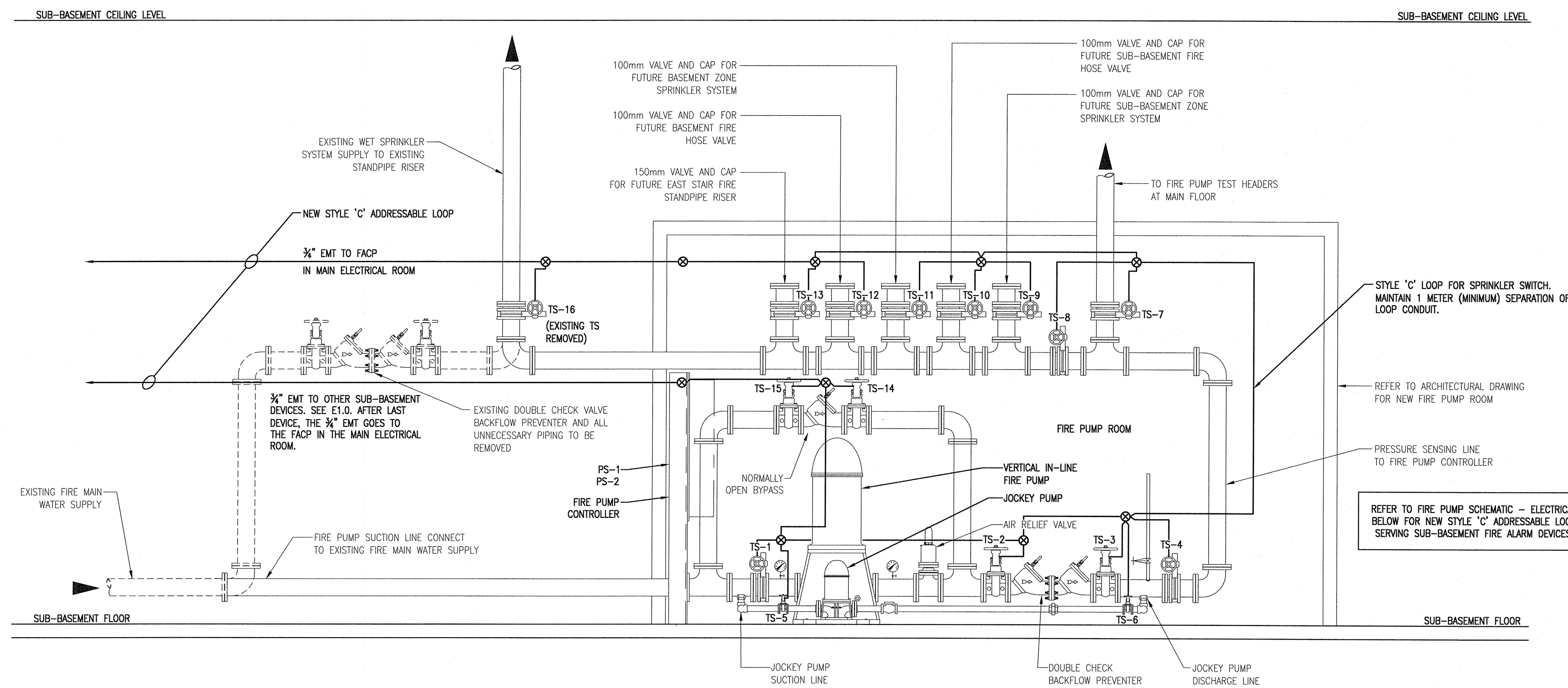
2 FIRE PUMP SCHEMATIC - ELECTRICAL (REFER TO PLAN ON E1.0) E3.0 SCALE: NTS
