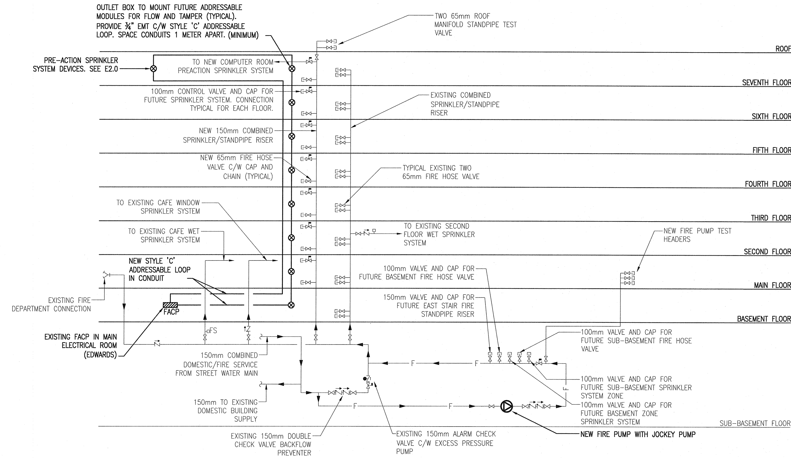
1 SPRINKLER SYSTEM SCHEMATIC RISER DIAGRAM - ELECTRICAL E3.0 SCALE: NTS
