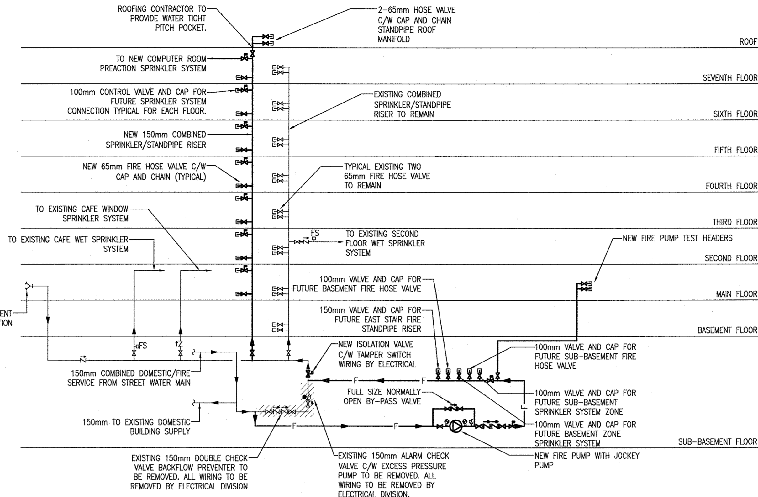
2 SPRINKLER SYSTEM SCHEMATIC RISER DIAGRAM FP-3 SCALE: NOT TO SCALE
