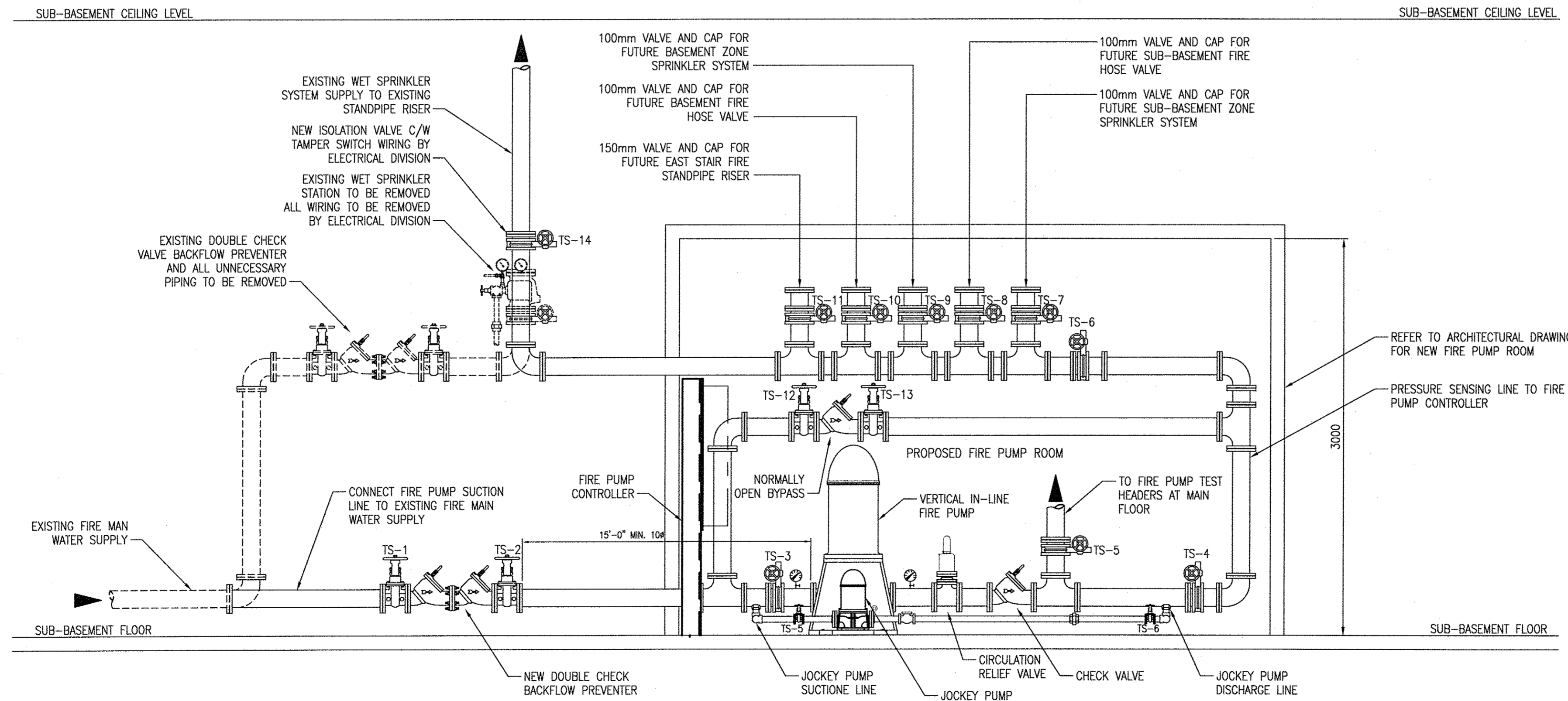
3 FIRE PUMP ROOM SECTION FP-3 SCALE: 1:30
