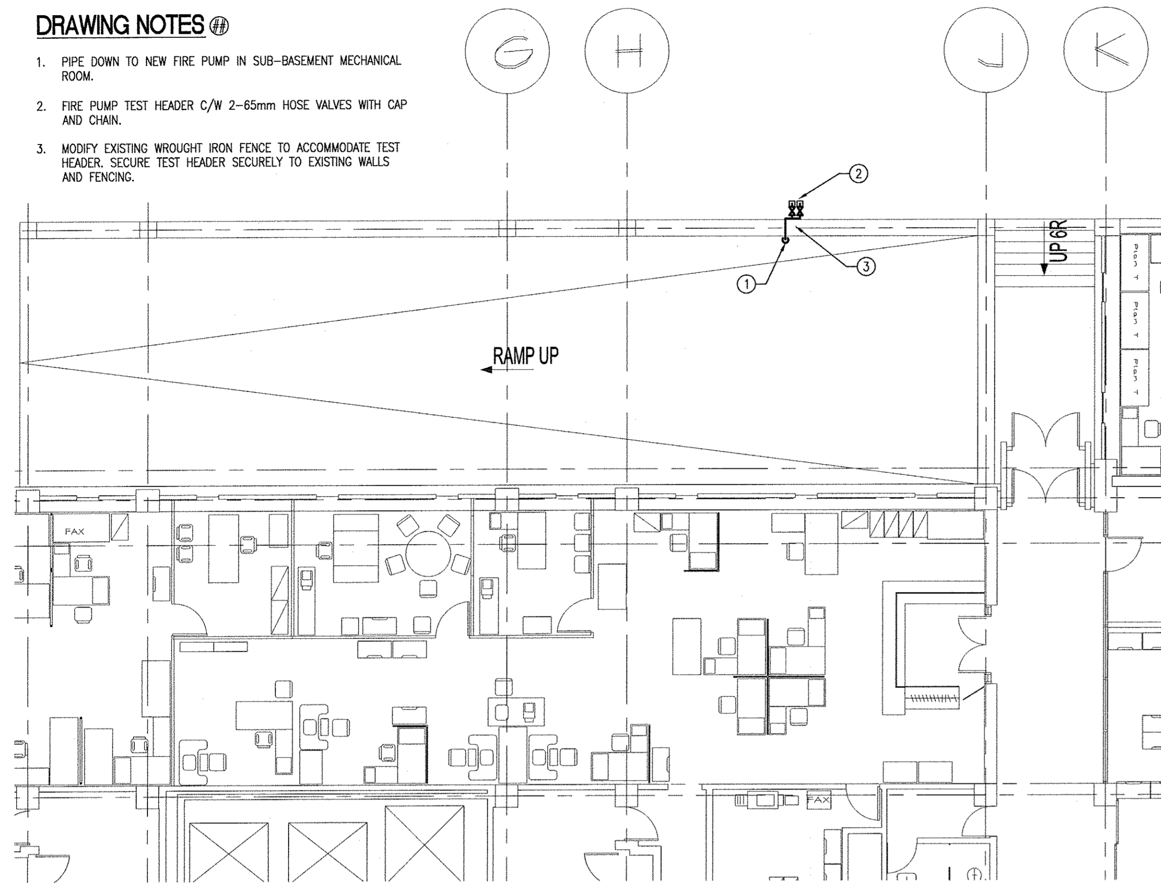
1 PART MAIN FLOOR PLAN - FIRE PROTECTION FP-3 SCALE: 1:100
