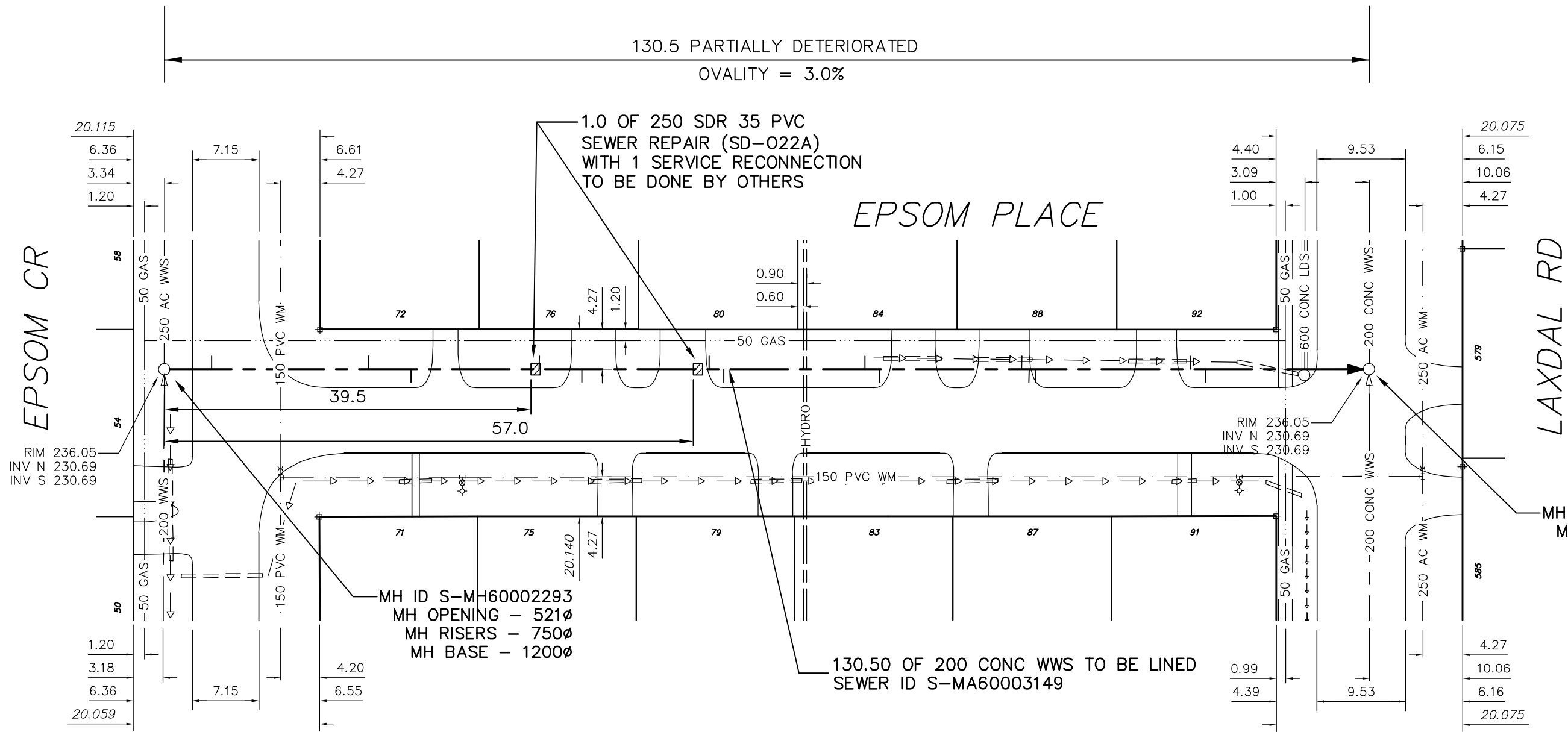
SEWER JUNCTION INFORMATION FROM SEWER VIDEO INSPECTION S-MA60003149
