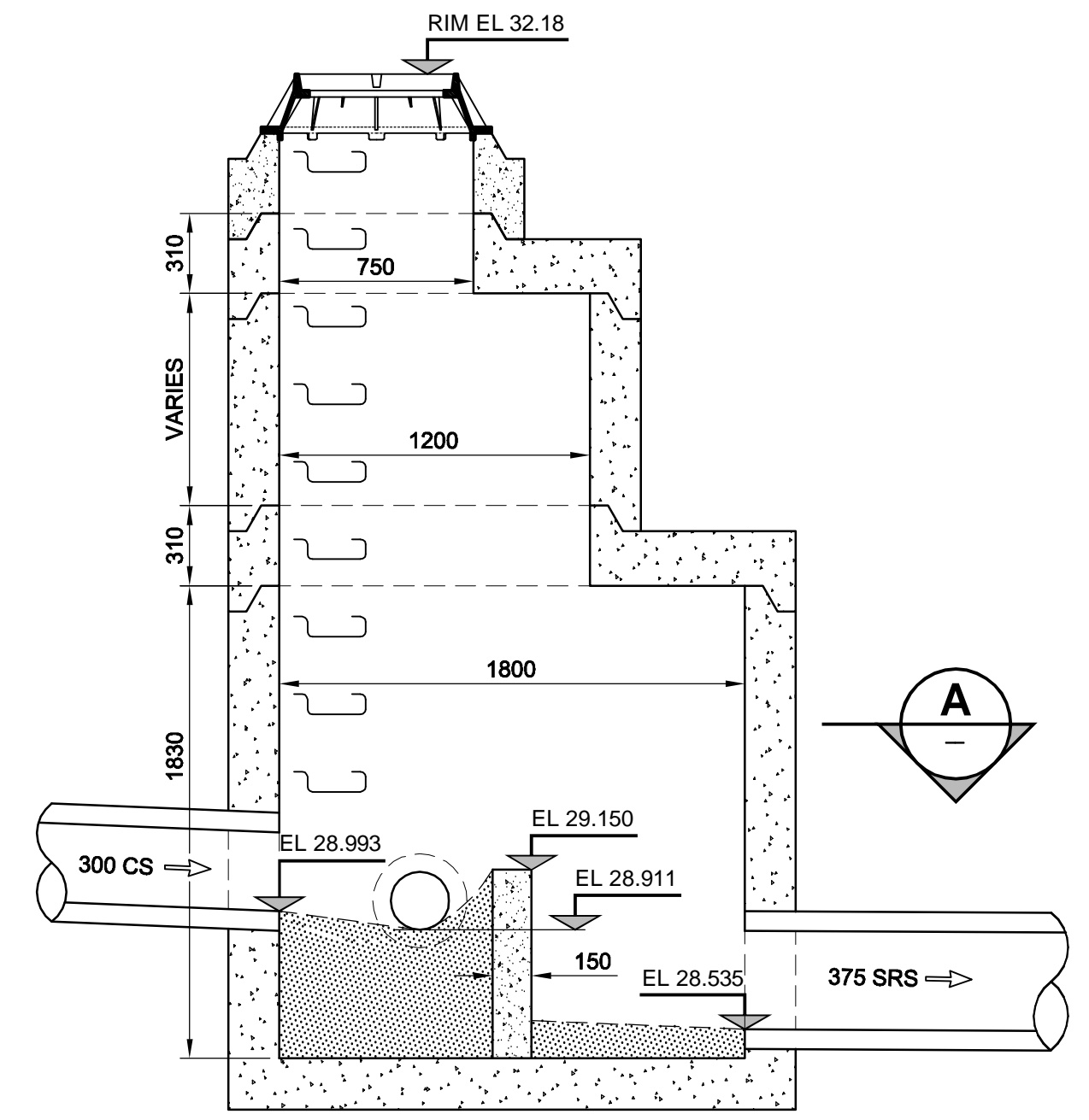
MANHOLE 1 OVERFLOW DETAIL
