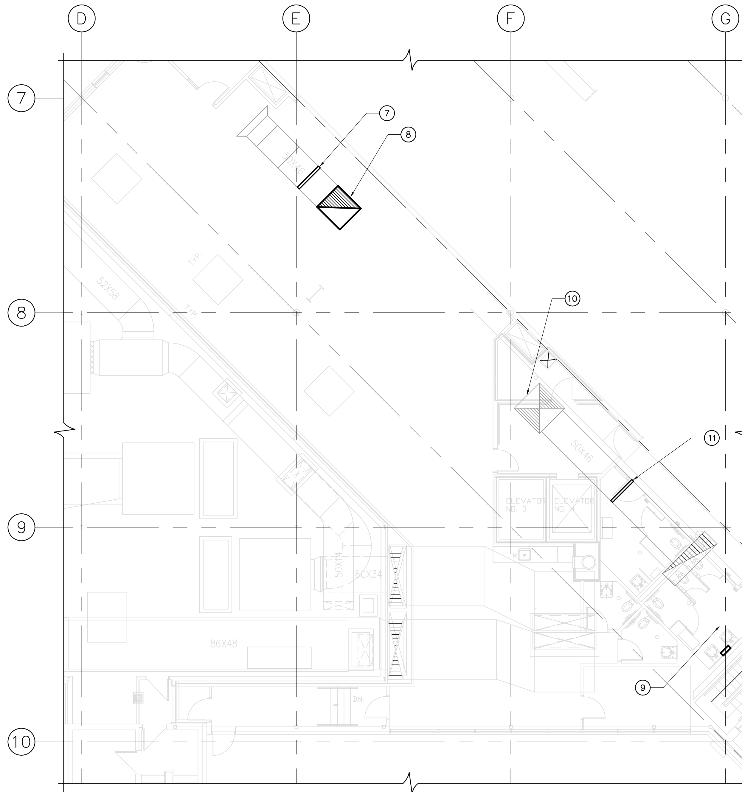
FOURTH FLOOR HVAC PLAN SCALE: 1/8"=1'-0"
