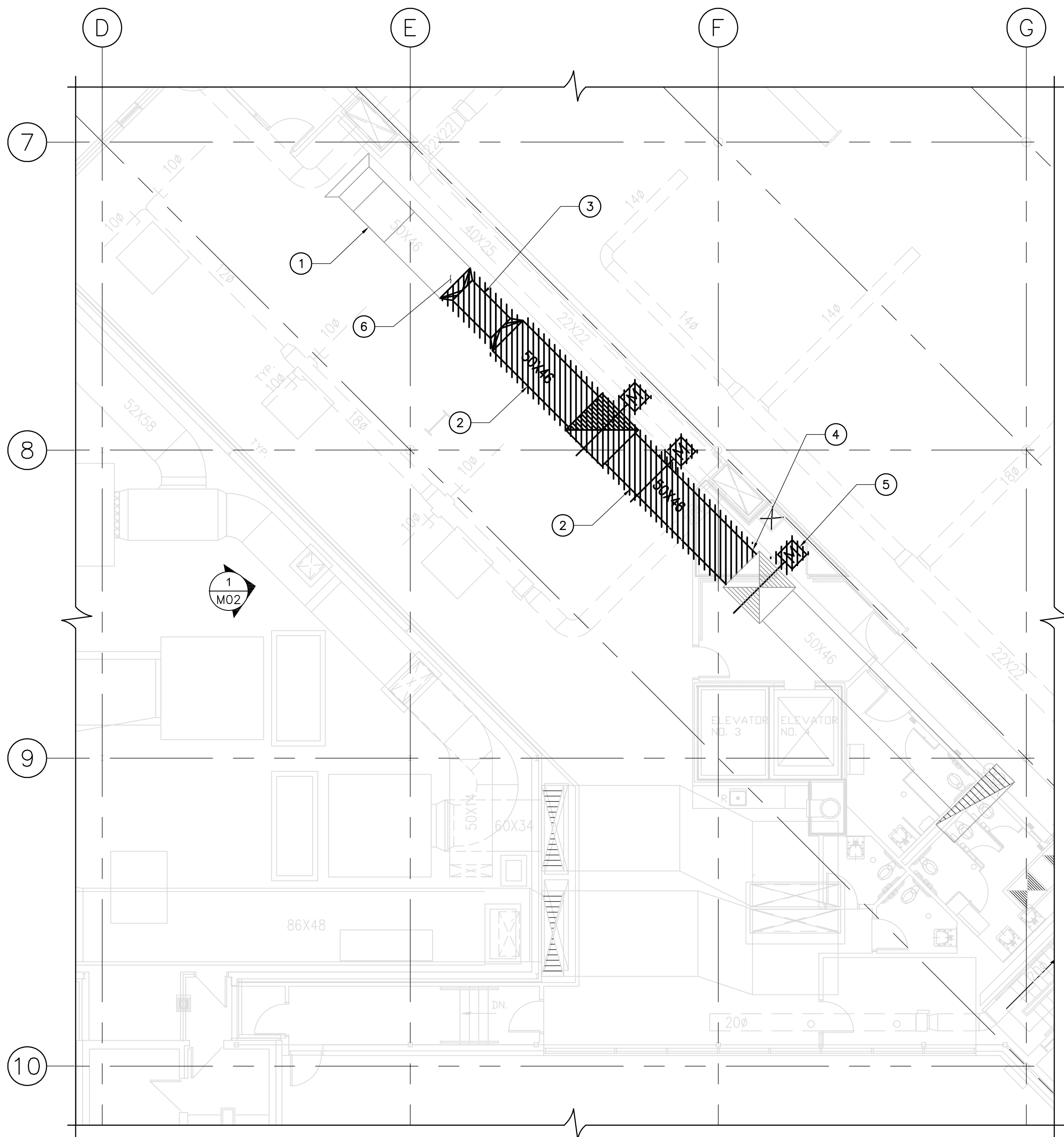
FOURTH FLOOR HVAC DEMOLITION PLAN SCALE: 1/8"=1'-0"
