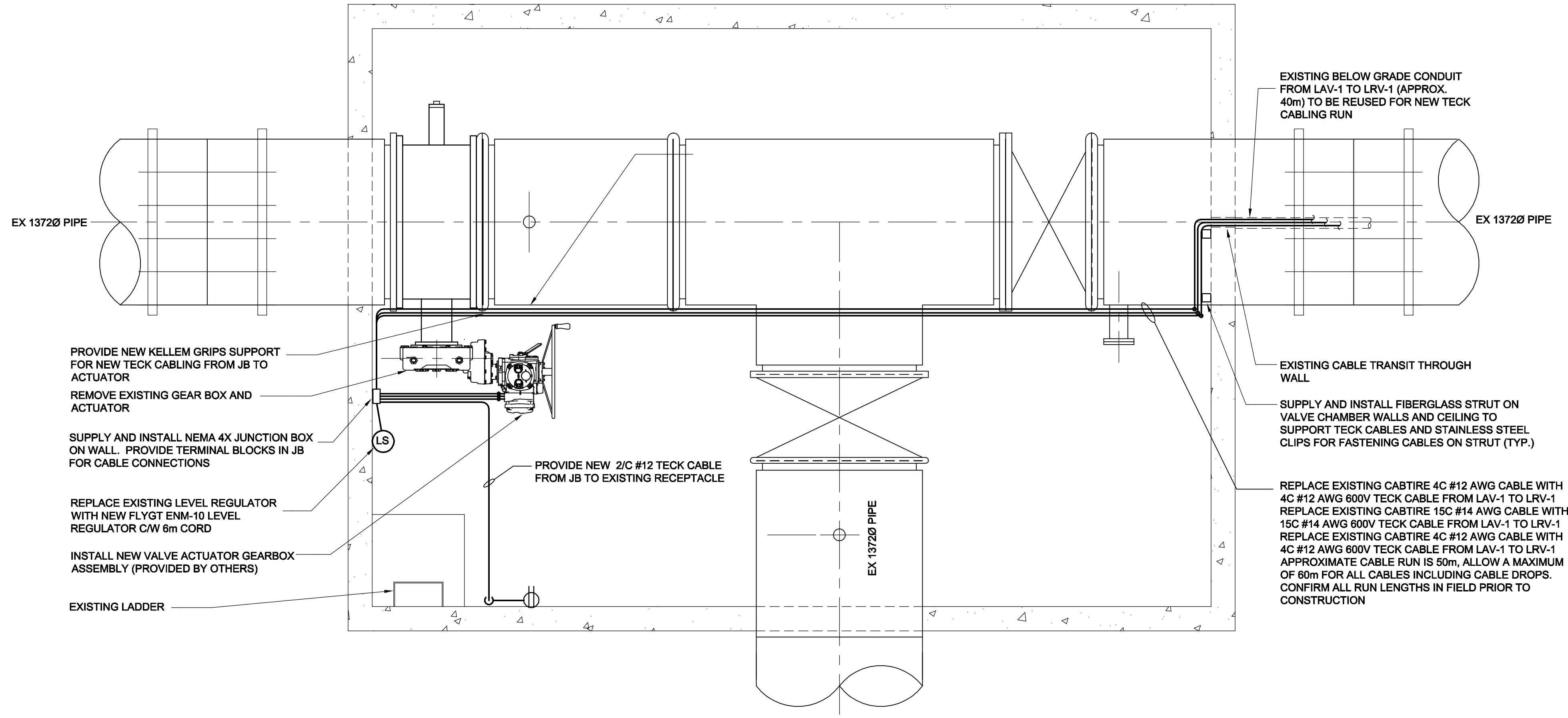
VALVE CHAMBER LAV1 SCALE 1:25 0 0.25 0.5 0.75 m
