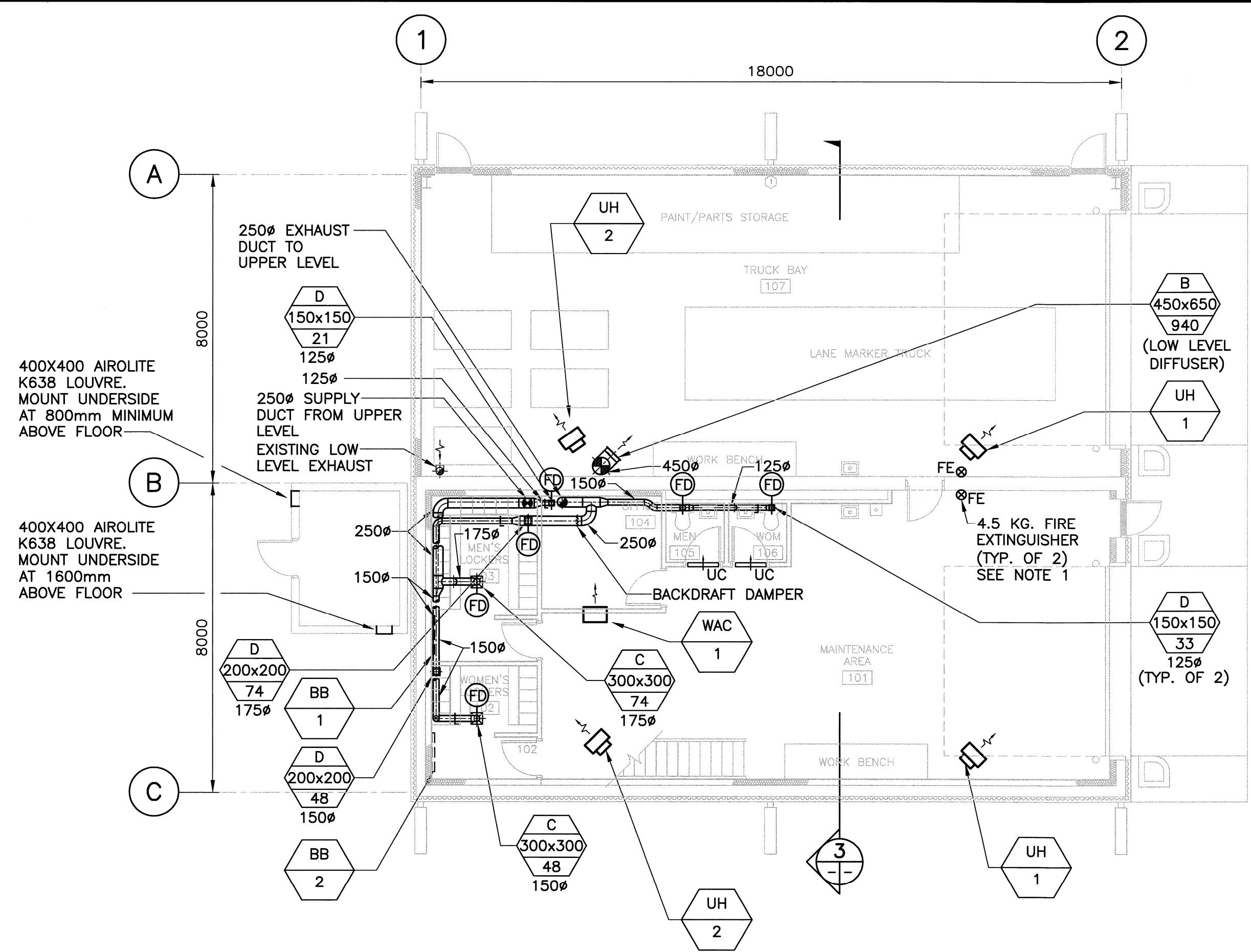
2 FLOOR PLAN (LOW LEVEL) - VENTILATION 1:100
