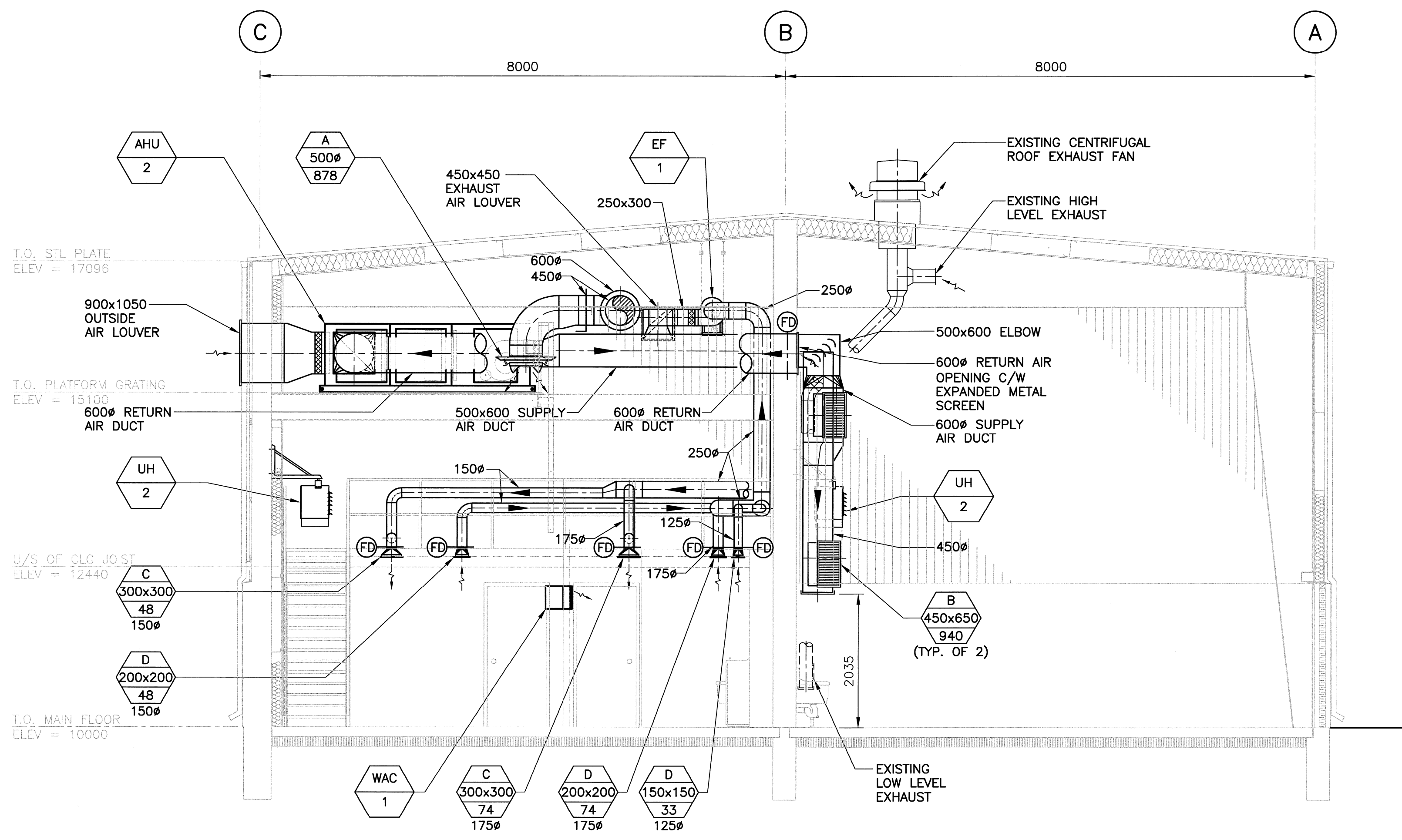
3 SECTION 1:50
