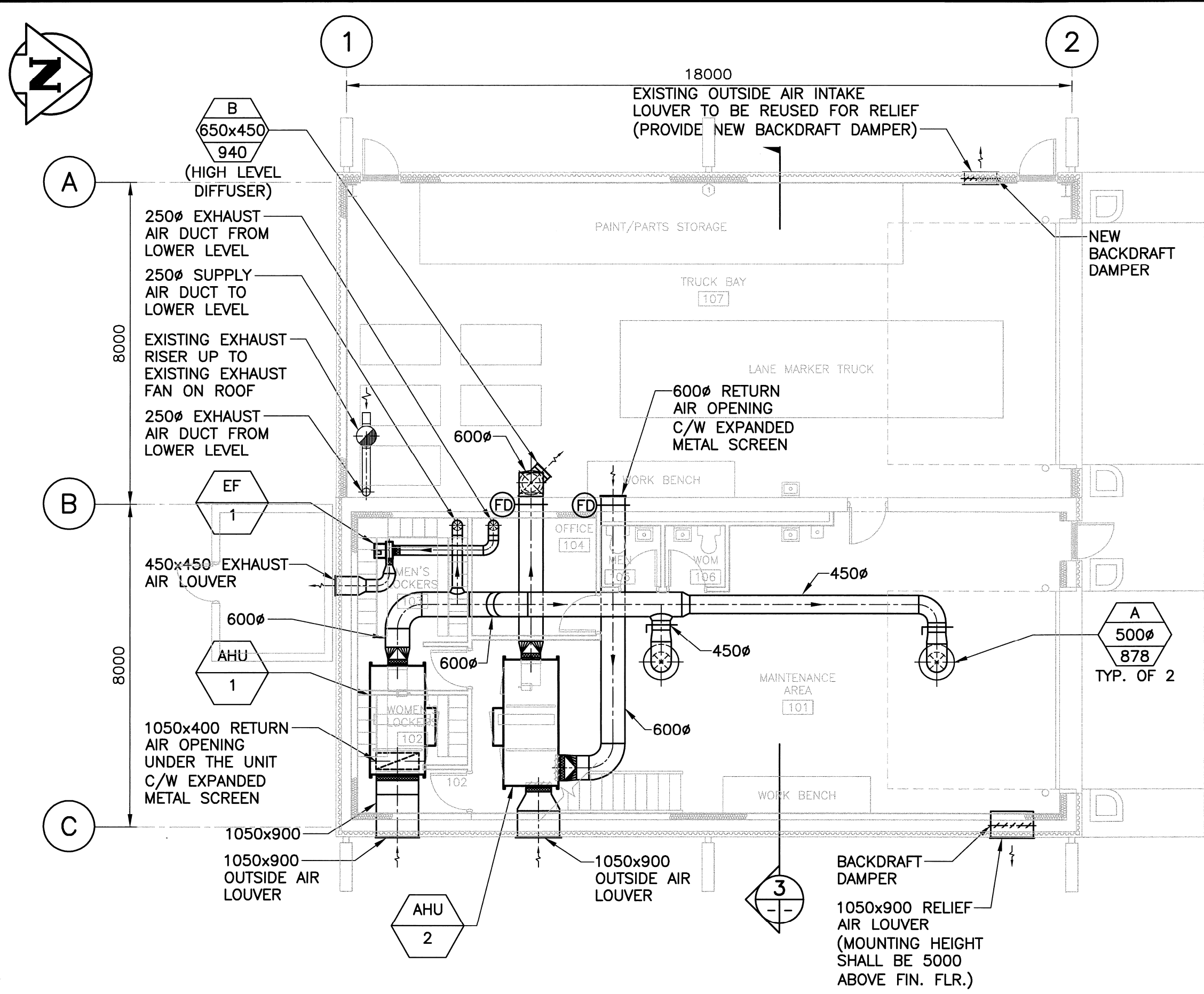
1 FLOOR PLAN (HIGH LEVEL) - VENTILATION 1:100
