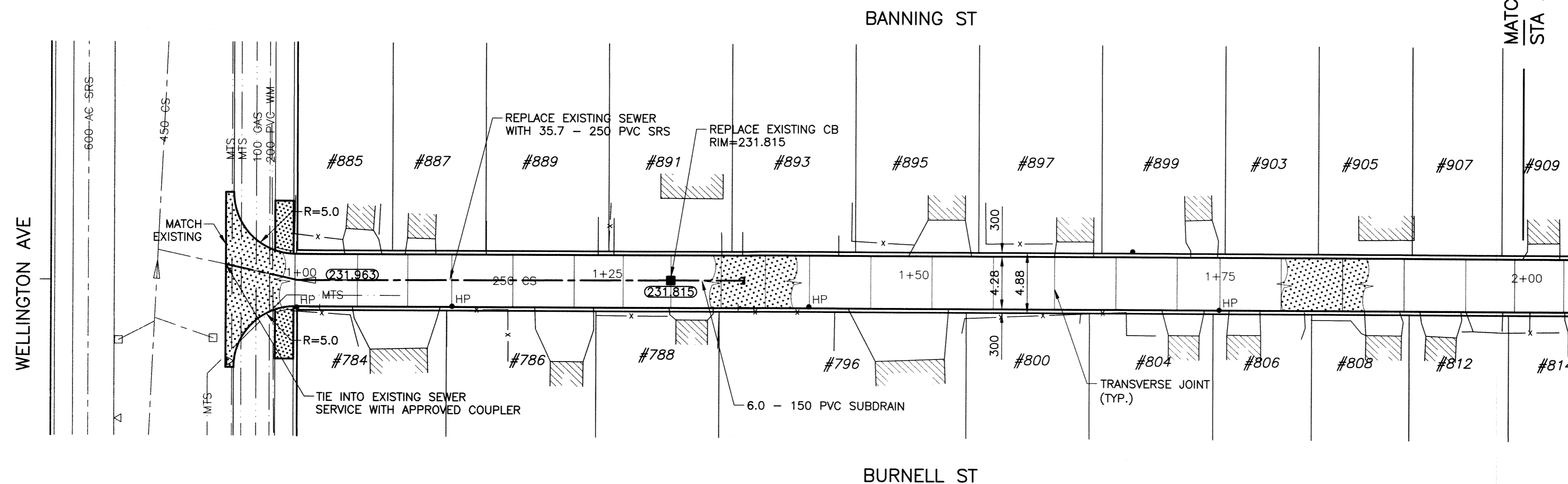
ALLEY PAVEMENT PLAN
