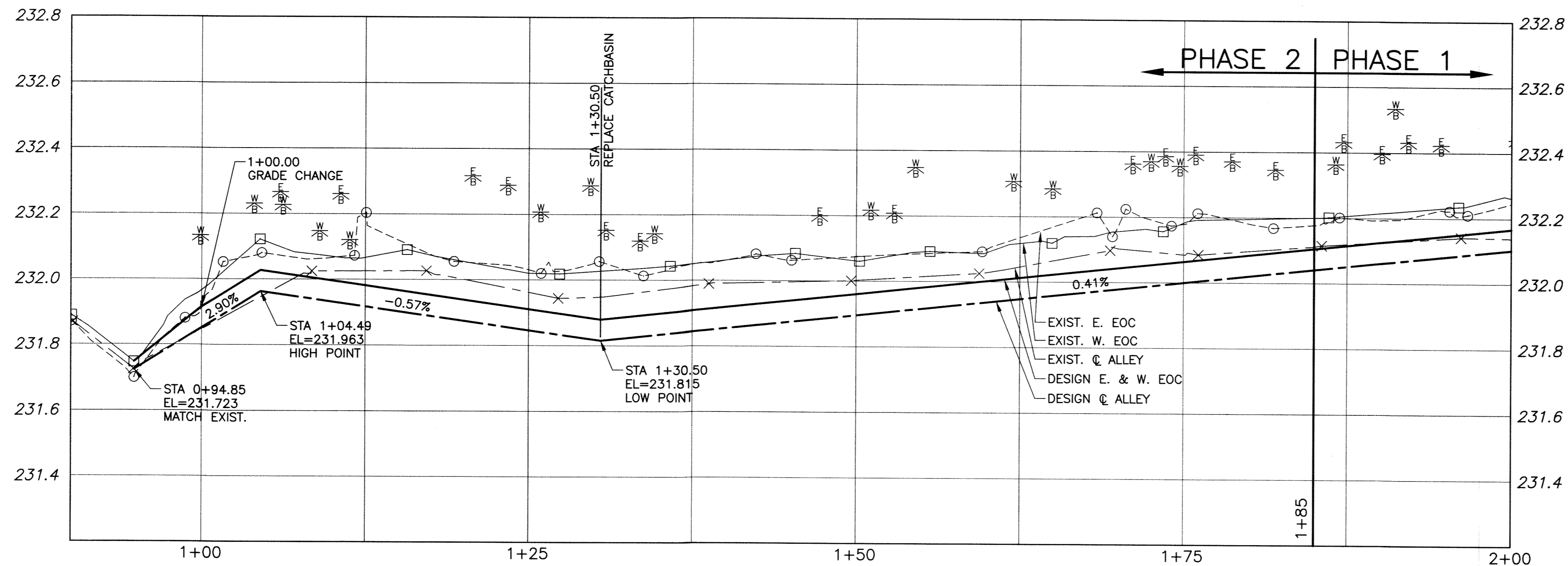
ALLEY PAVEMENT PROFILE
