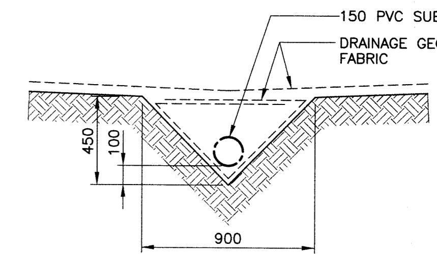
SUBDRAIN DETAIL
