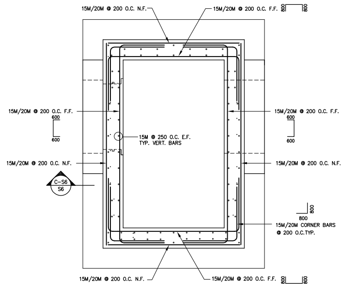
SECTION A-S6/S6 1:25
