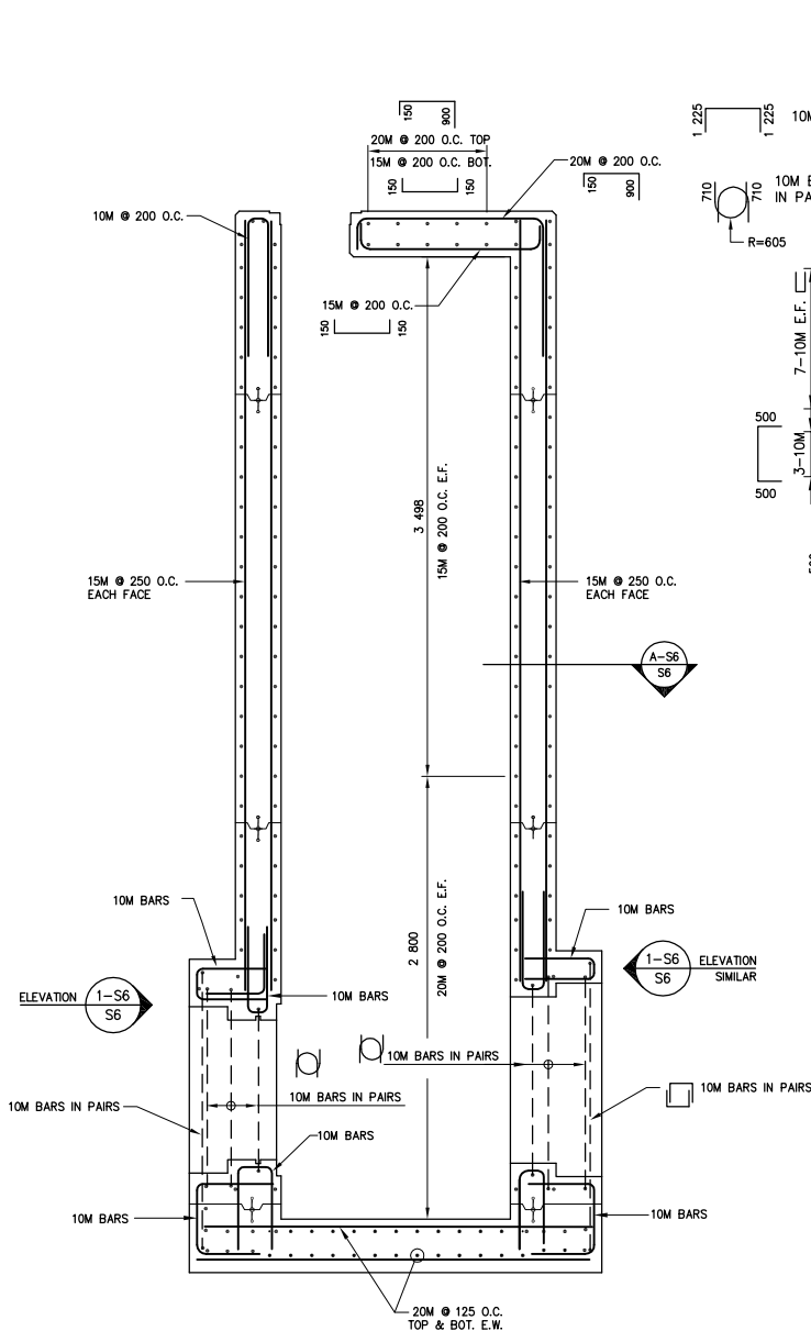
SECTION B-S6/S6 1:25
