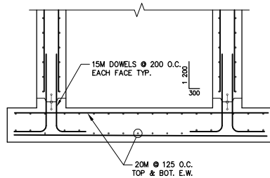
SECTION C-S6/S6 1:25
