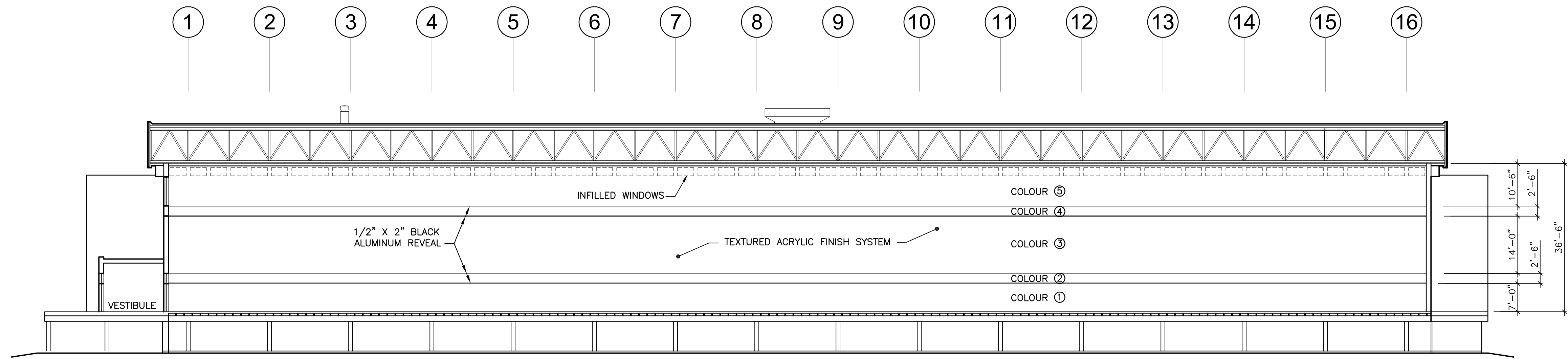
1 INTERIOR ELEVATION (NORTH) SCALE: 1/16"=1'-0"
