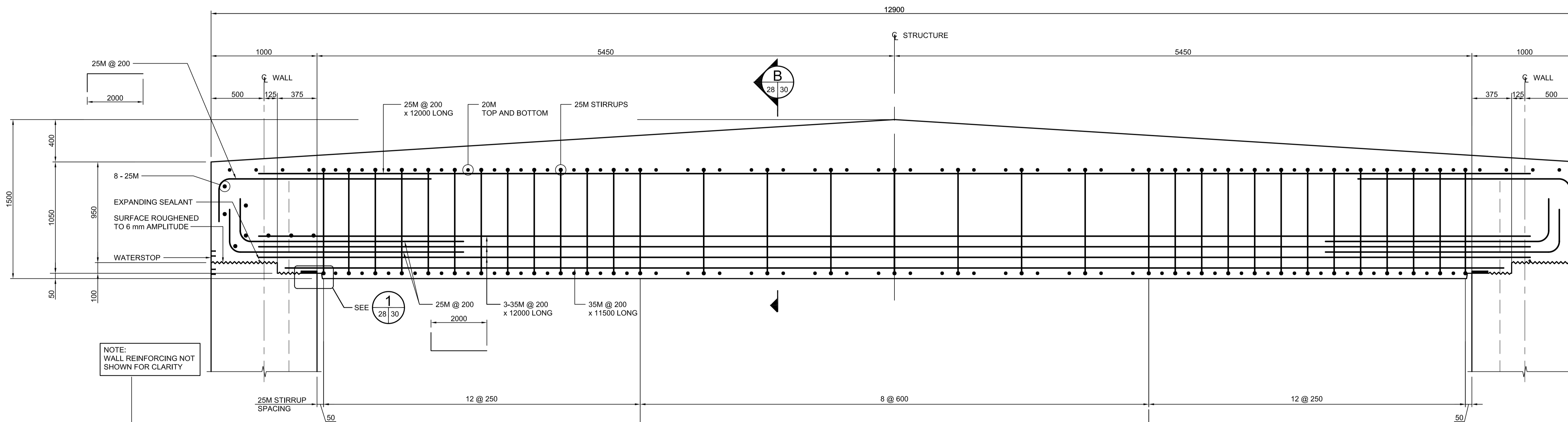
SEGMENT TYPE B SCALE 1:20
