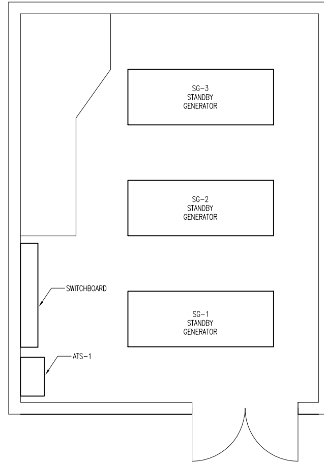
GENERATOR ROOM
