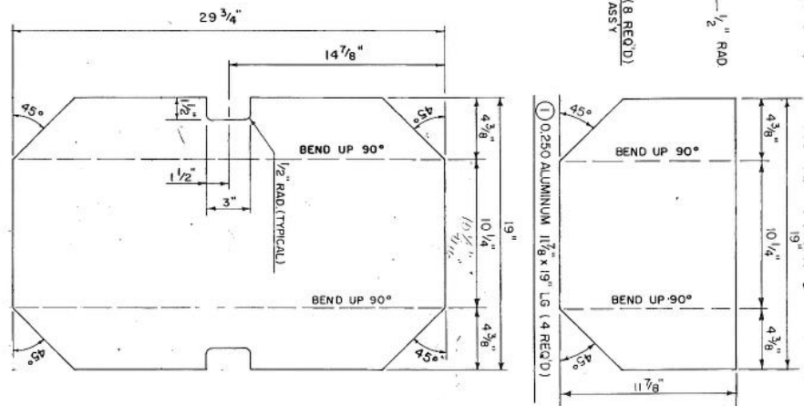
② 0.250 ALUMINIUM 19" x 29 3/4" LG (2 REQ'D)
