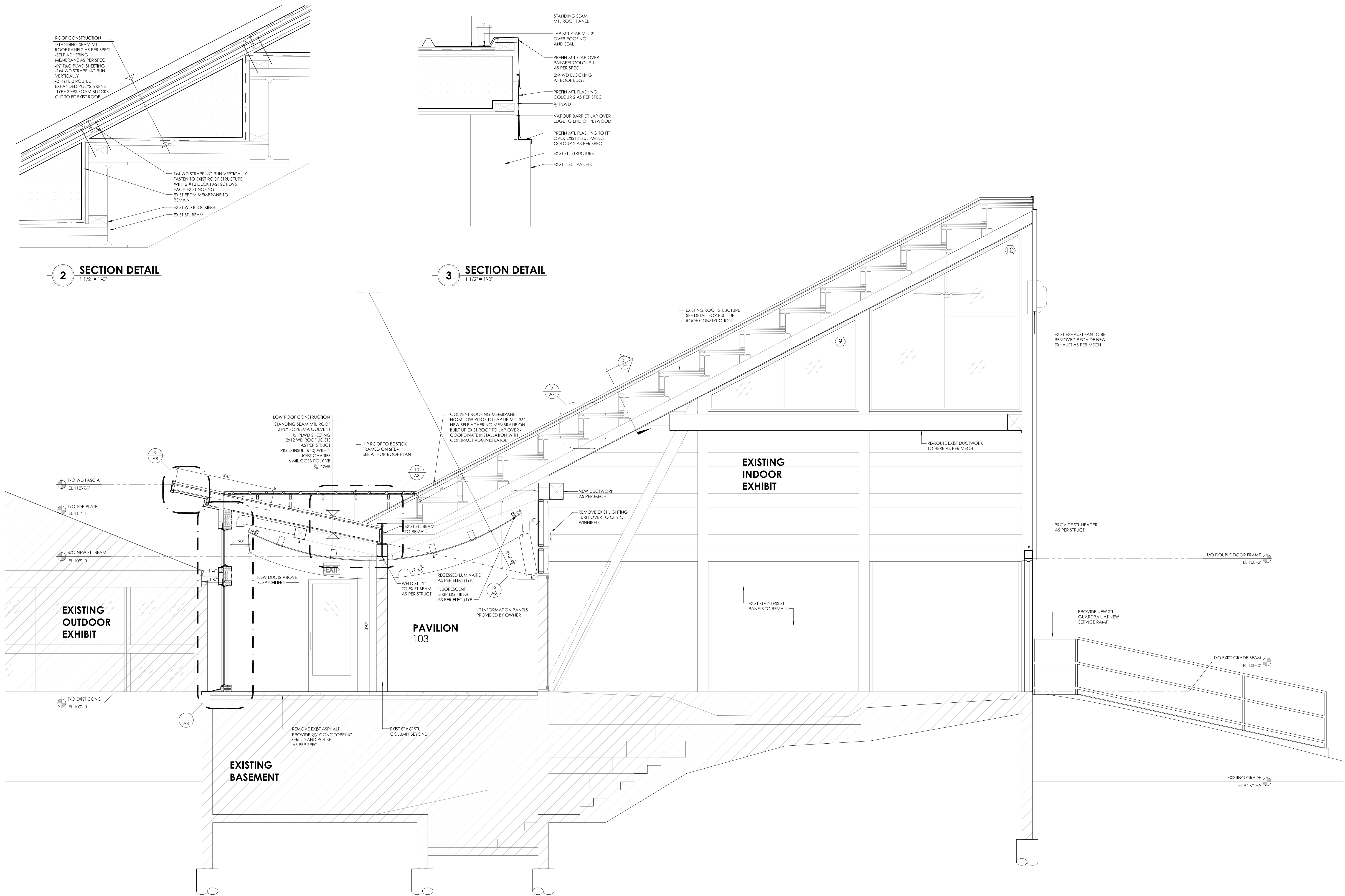
1 BUILDING SECTION 3/8" = 1'-0"
