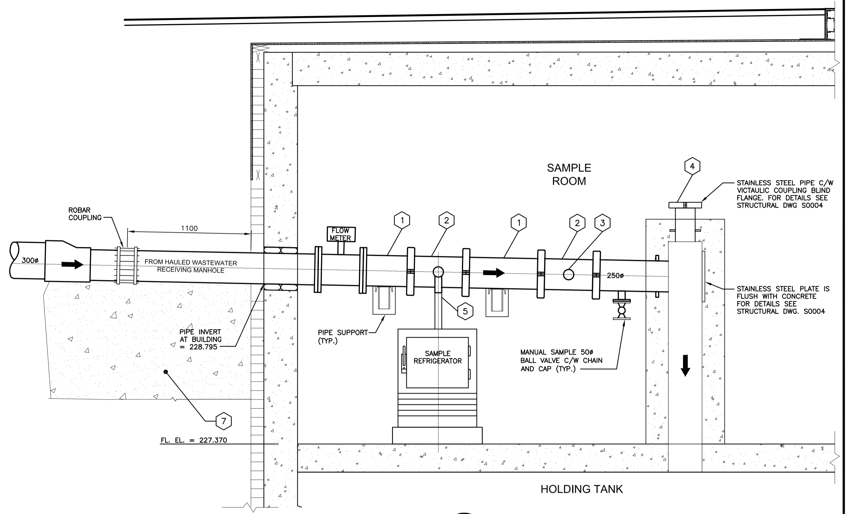
A SECTION P0002 1:20
