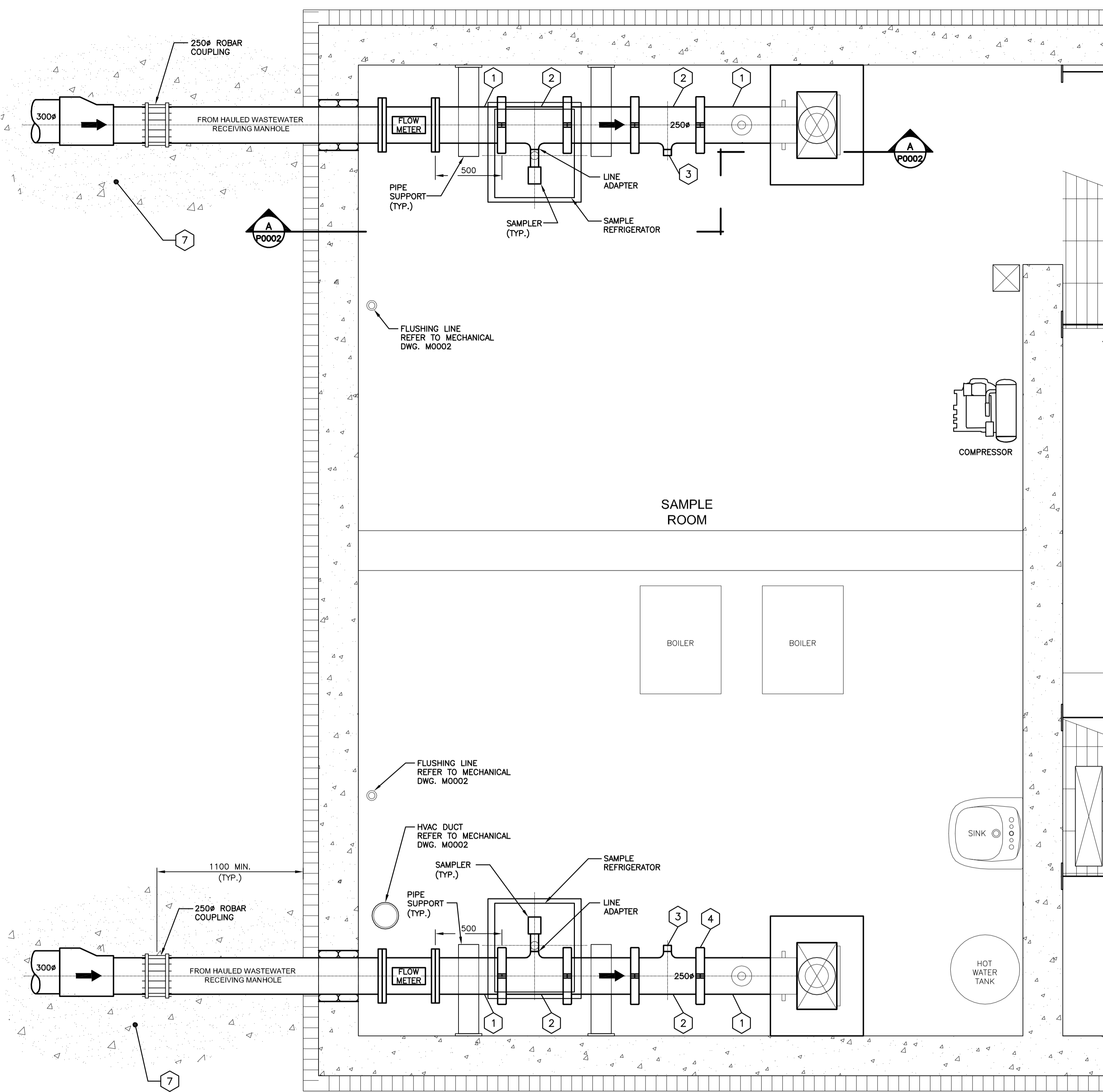
1 PLAN P0002 1:20
