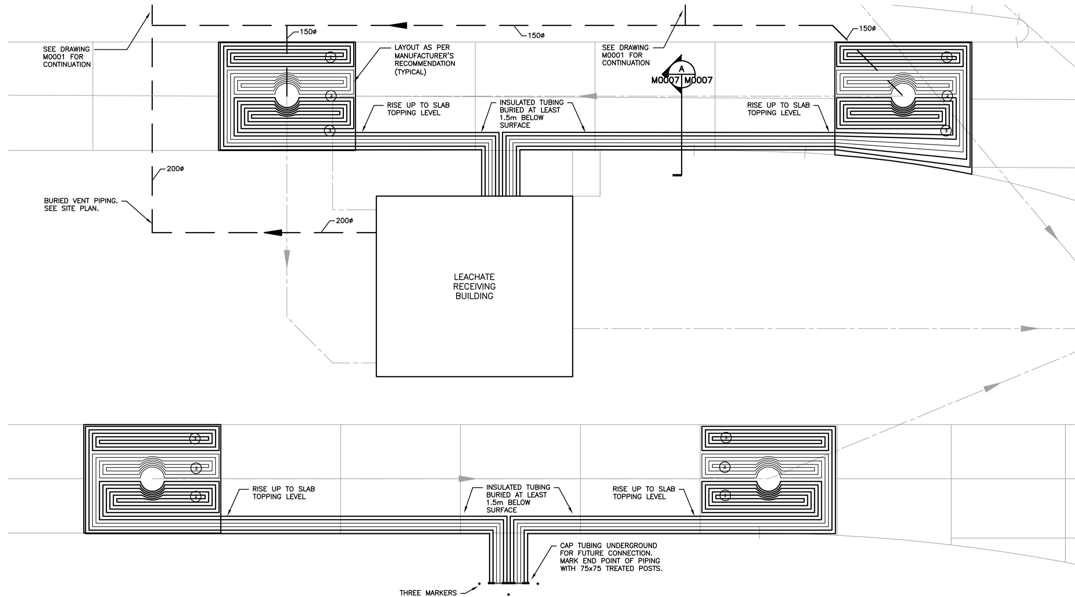
1 MECHANICAL SITE PLAN M0007 1:100
