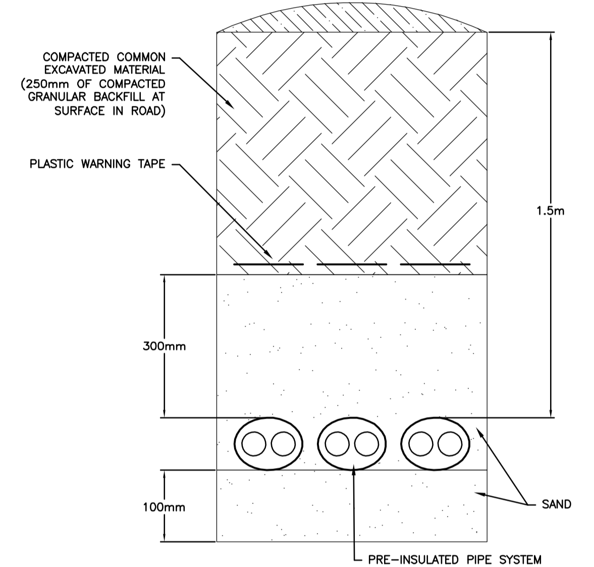
A BURIED HYDRONIC PIPING M0007 NTS
