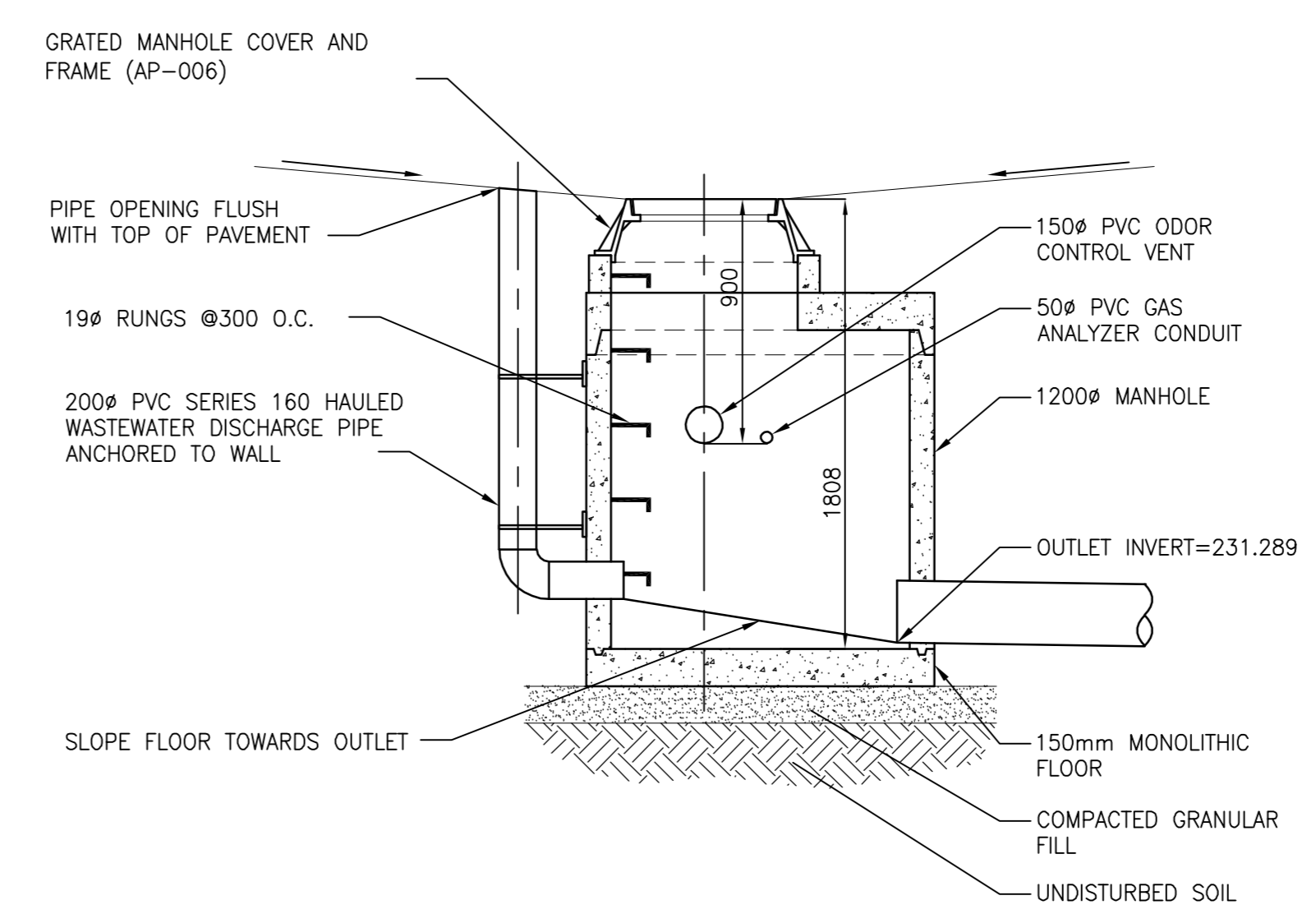
2 RECEIVING MANHOLE DETAIL C0007 1:25
