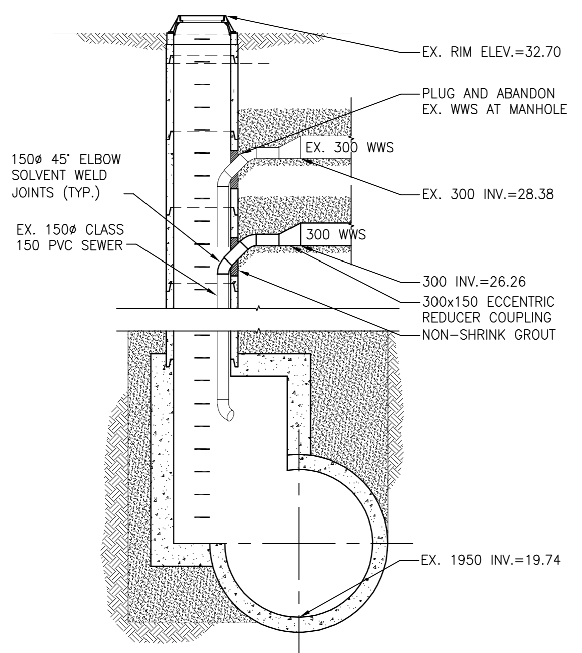
1 INTERCEPTOR SEWER CONNECTION DETAIL C0007 1:50
