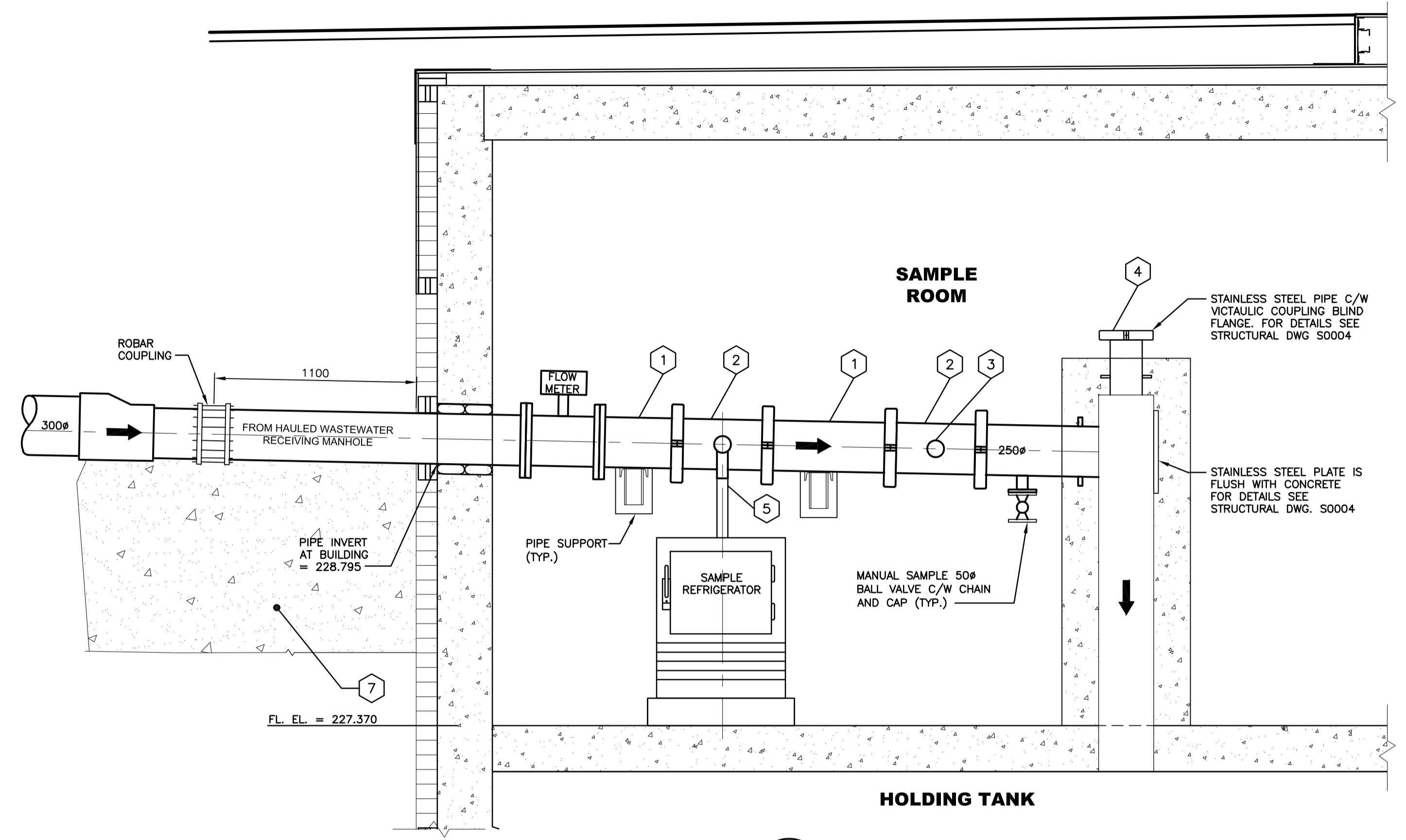
A SECTION P0002 1:20
