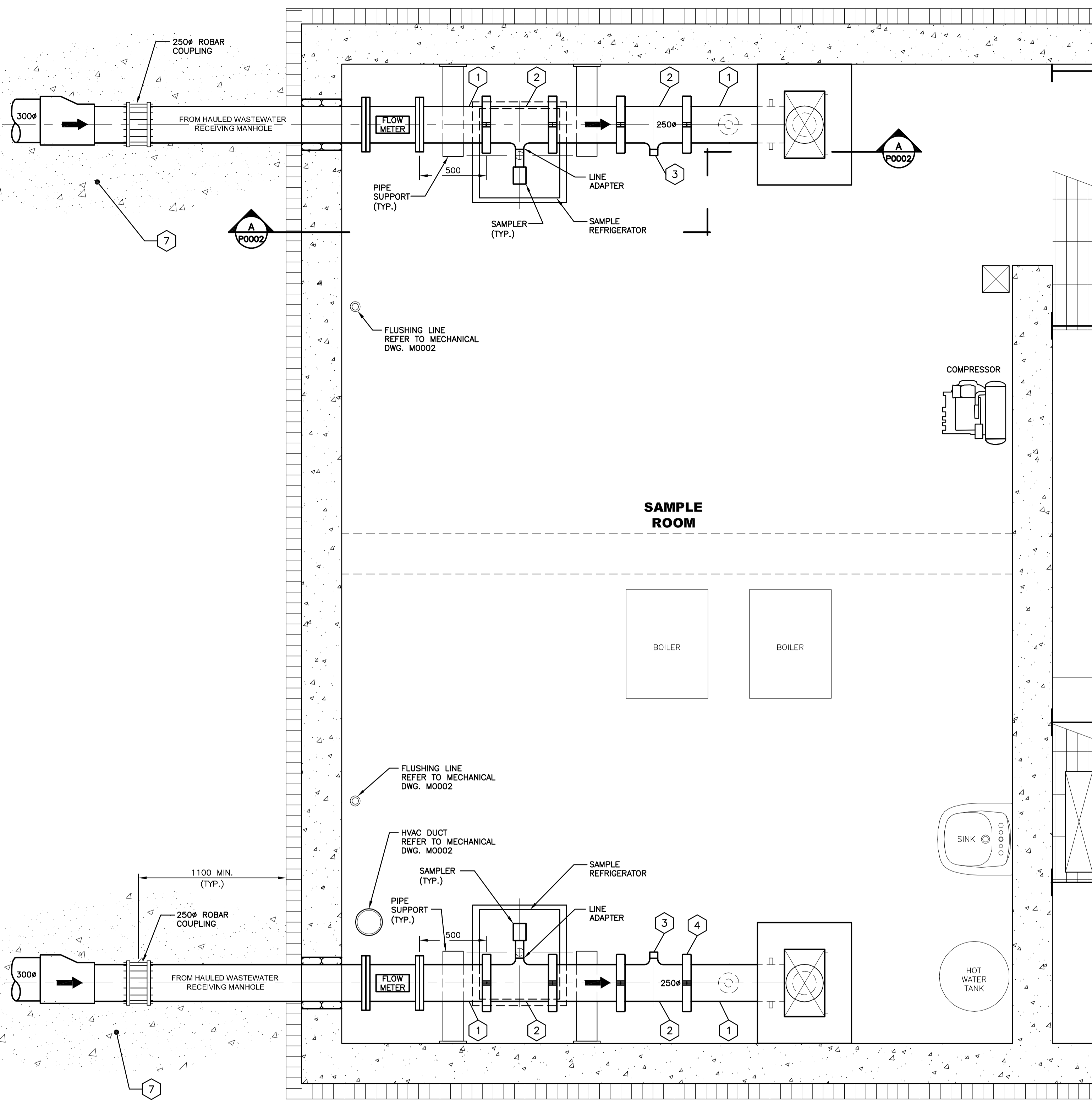
1 PLAN P0002 1:20
