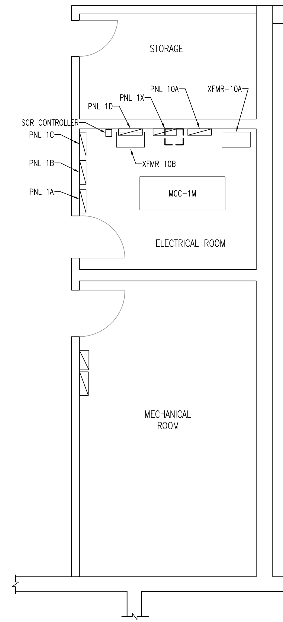
ADMINISTRATION BUILDING ELECTRICAL ROOM 1:50
