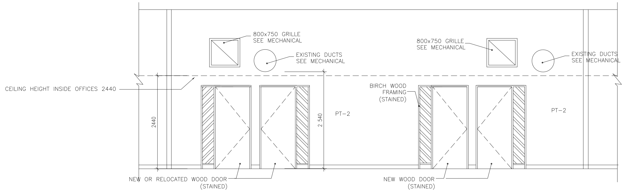
1 A10 EXTERIOR ELEVATION OFFICES 1:50
