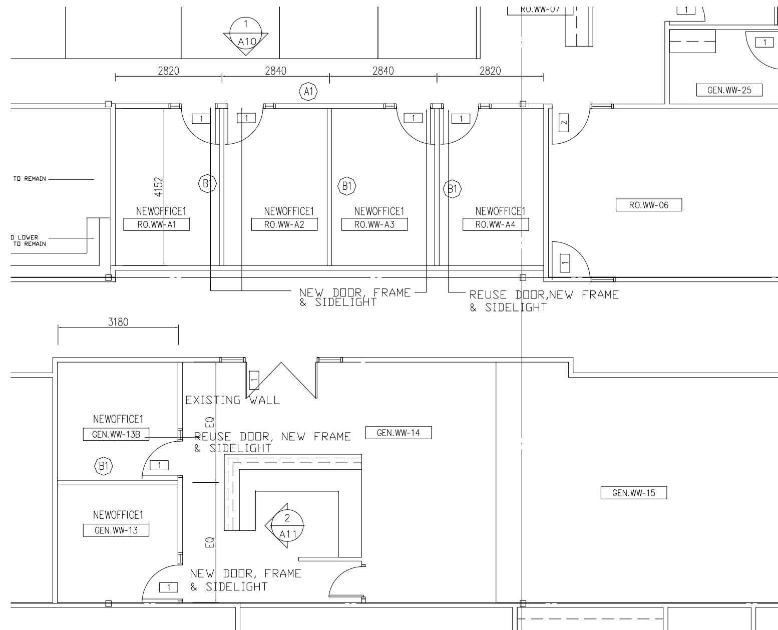
FLOOR PLAN AREA B
