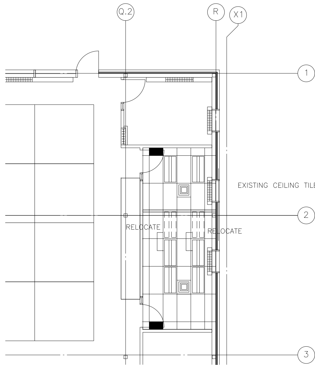
REFLECTED CEILING PLAN AREA C
